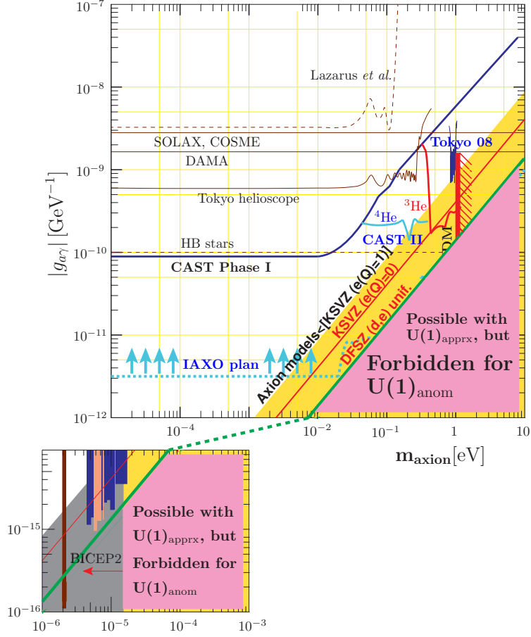
FIG. 2: The allowed parameter space of g_{a\gamma\gamma} [\text{GeV}^{-1}] = 1.57 \cdot 10^{-10} c_{a\gamma\gamma} vs. axion mass. The lavender part is not allowed if the U(1)_{\text{PQ}} is the anomalous U(1)_{\text{anom}} . However, it can be allowed for some approximate U(1)_{\text{PQ}} , as shown in Ref. [34] for the flipped-SU(5) model of Ref. [35].
