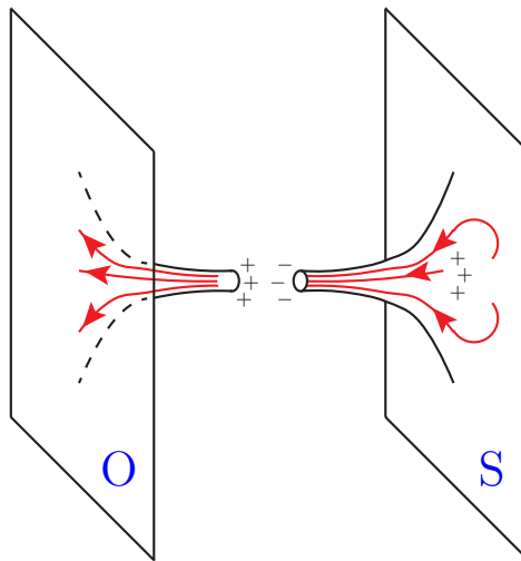
FIG. 1: Escaping charges through a wormhole.
