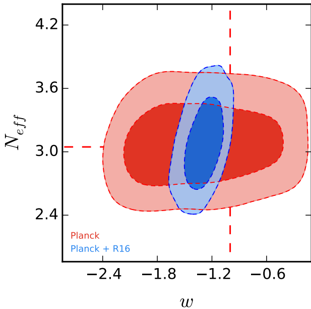
Figure 1. Constraints at 68% and 95% c.l. on the N_{eff} vs w plane assuming the Planck data set with and without the R16 prior on H_0 . As one can see, when the R16 prior is included, a preference for w < -1 is clearly present, while N_{eff} is consistent with the standard expectations. An extended \Lambda CDM theoretical framework of 12 parameters is assumed in the analysis.
