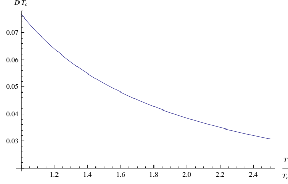
Figure 1: DT_c vs. \frac{T}{T_c} for T \geq T_c
