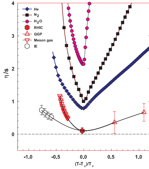
Figure 3: \frac{\eta}{s} vs. \frac{T-T_c}{T_c} reproduced from [41].
