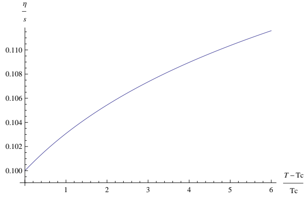
Figure 2: \frac{\eta}{s} vs. \frac{T-T_c}{T_c} for T \geq T_c assuming \frac{\eta}{s}|_{T=T_c} = 0.1
