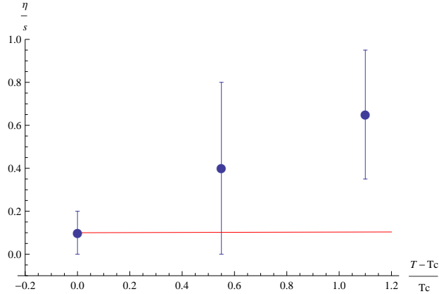
Figure 4: Combined plots of Figures 2 and 3: the graph in red is from Figure 2 (our calculations) and the set of three points with error bars are from Figure 3 (RHIC QGP data from [41]).
