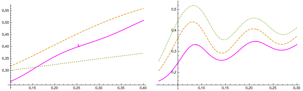
Figure 2. Relative differences between equilibrium solutions and \dot{\theta}/T , normalized to \dot{\theta}/T . Left: as functions of \dot{\theta} for different t_{max} : \tau \equiv t_{max}T = 30 (thick); 10 (dashed); 3 (dotted); \ddot{\theta} = 0.1 . Right: as functions of \ddot{\theta} for different \dot{\theta} : \dot{\theta} = 0.1 (thick); 0.2 (dashed); 0.3 (dotted); \tau \equiv t_{max}T = 10 .
