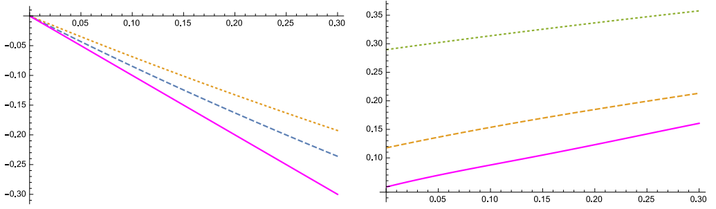
Figure 1. Left: \dot{\theta}/T for infinite time integration (thick line). Cut-off in time integration \tau \equiv t_{max}T = 10 (dashed); 3 (dotted). Right: relative differences between the equilibrium solutions and \dot{\theta}/T , normalized to \dot{\theta}/T , as functions of \dot{\theta} for different t_{max} : \tau \equiv t_{max}T = 30 (thick); 10 (dashed); 3 (dotted).
