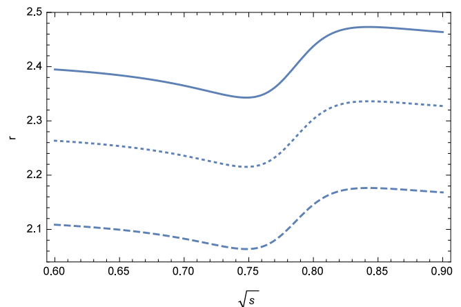
FIG. 5. r as a function of \sqrt{s} for different CKM matrix elements. The dash line, dot line and solid line corresponds to the maximum, middle, and minimum CKM matrix element for the decay channel of B_c^+ \rightarrow D^+ \pi^+ \pi^- , respectively.
