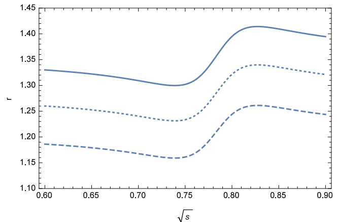
FIG. 6. r as a function of \sqrt{s} for different CKM matrix elements. The dash line, dot line and solid line corresponds to the maximum, middle, and minimum CKM matrix element for the decay channel of B_c^+ \rightarrow D_s^+ \pi^+ \pi^- , respectively.
