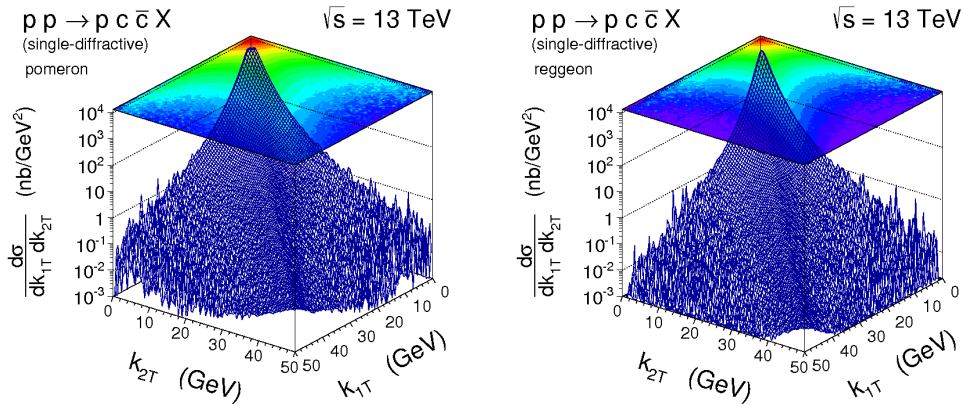
Figure 4: Double differential cross sections as a function of initial gluons transverse momenta k_{1T} and k_{2T} for single-diffractive production of charm at \sqrt{s} = 13 TeV. The left and right panels correspond to the pomeron and reggeon exchange mechanisms, respectively.
