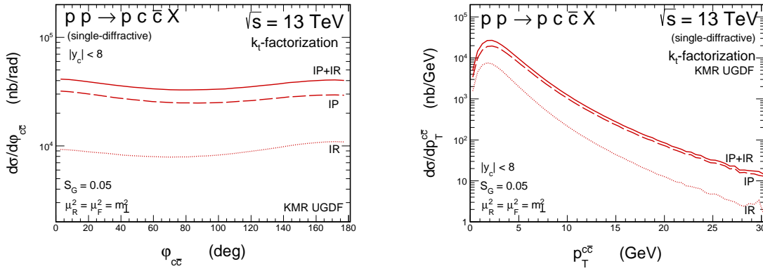
Figure 3: The distribution in \phi_{c\bar{c}} (left panel) and distribution in p_T^{c\bar{c}} (right panel) for k_t -factorization approach at \sqrt{s} = 13 TeV.
