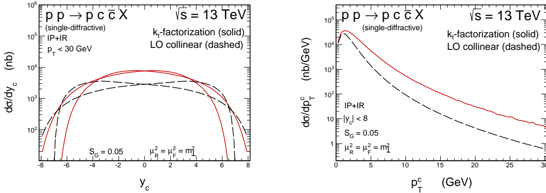
Figure 2: Rapidity (left panel) and transverse momentum (right panel) distributions of c quarks (antiquarks) for a single-diffractive production at \sqrt{s} = 13 TeV. Components of the g(IP)-g(p) , g(p)-g(IP) , g(IR)-g(p) , g(p)-g(IR) mechanisms are shown.
