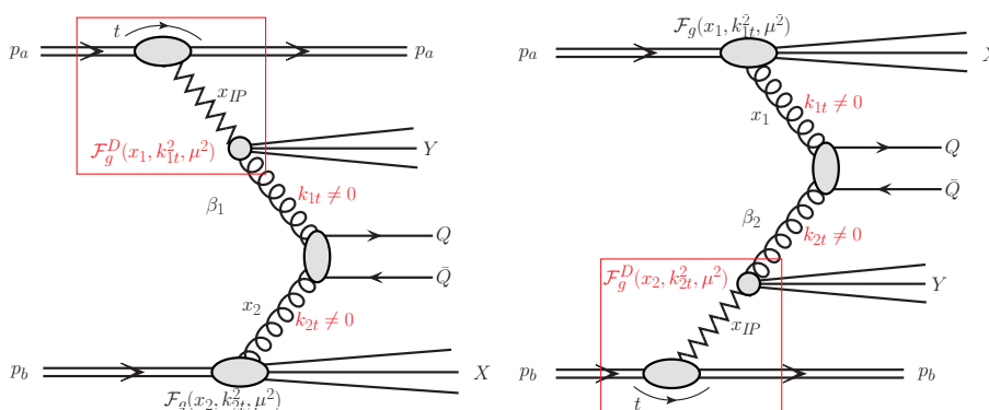
Figure 1: A diagrammatic representation for single-diffractive production of heavy quark pairs within the k_t -factorization approach.
