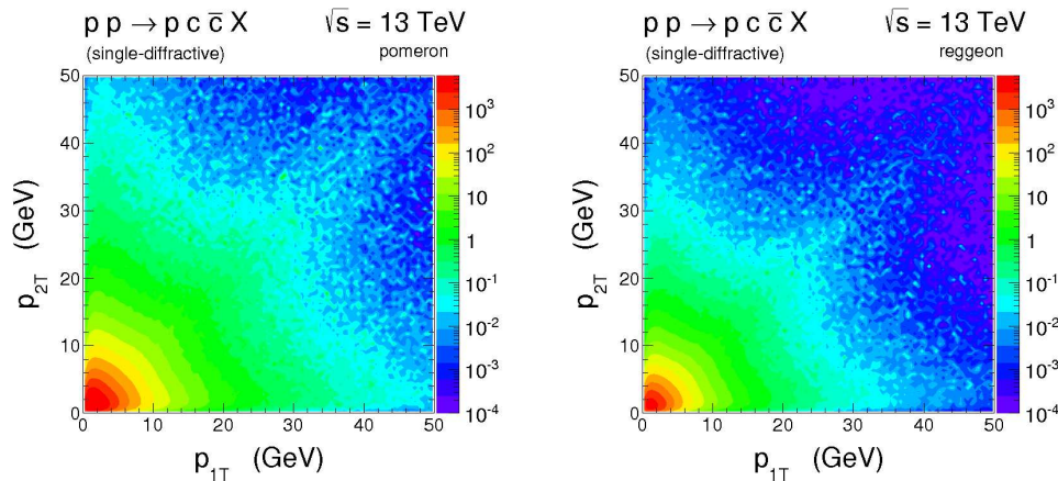
Figure 5: Double differential cross sections as a function of transverse momenta of outgoing c quark p_{1T} and outgoing \bar{c} antiquark p_{2T} for single-diffractive production of charm at \sqrt{s} = 13 TeV. The left and right panels correspond to the pomeron and reggeon exchange mechanisms, respectively.
