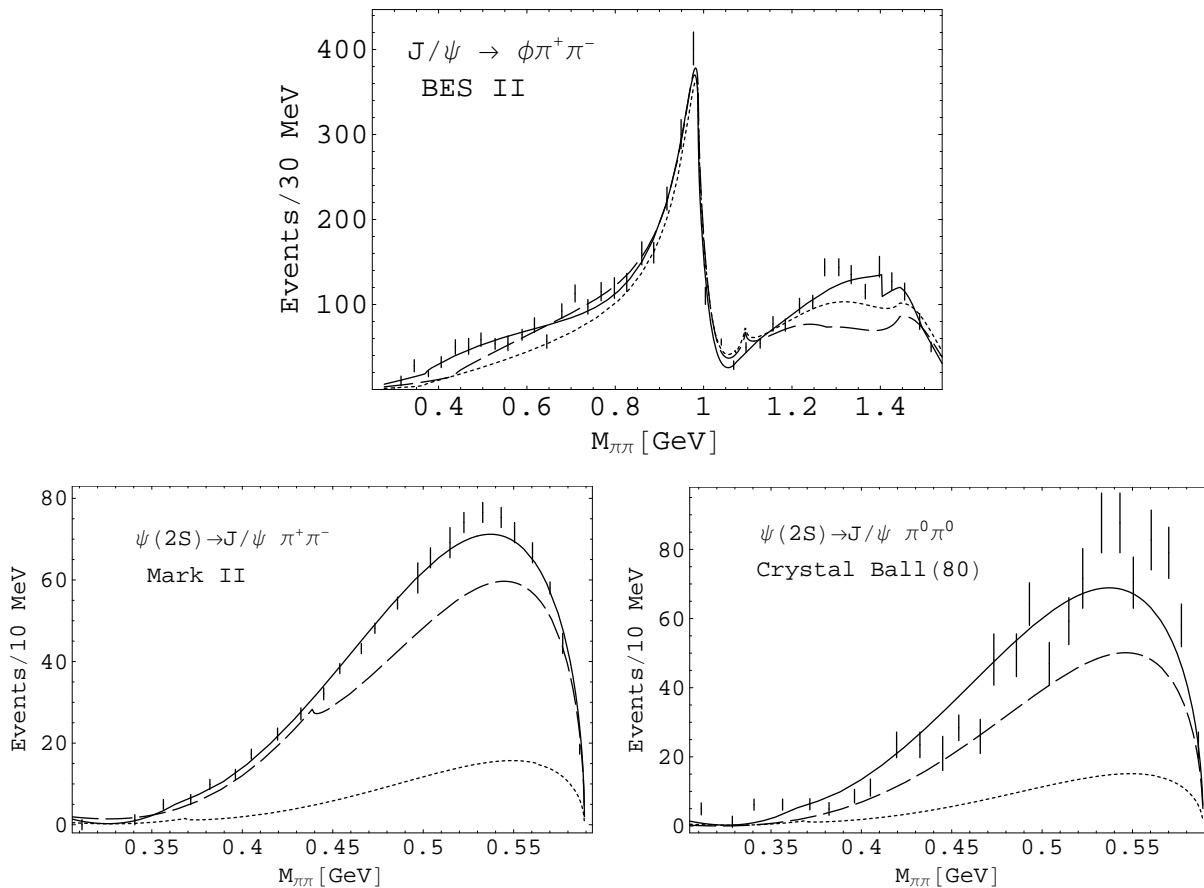
FIG. 1: The decays J/\psi \rightarrow \phi\pi\pi and \psi(2S) \rightarrow J/\psi\pi\pi . The solid lines correspond to contribution of all relevant f_0 -resonances; the dotted, of the f_0(500) , f_0(980) , and f_0'(1500) ; the dashed, of the f_0(980) and f_0'(1500) .
