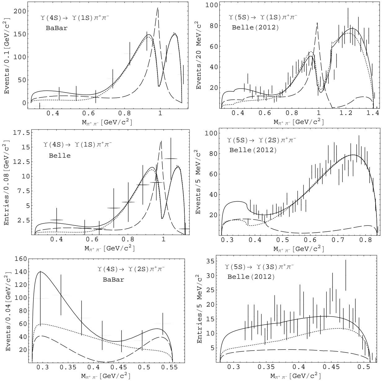
FIG. 3: The decays \Upsilon(4S) \rightarrow \Upsilon(1S, 2S)\pi^+\pi^- (left-hand) and \Upsilon(5S) \rightarrow \Upsilon(ns)\pi^+\pi^- ( n = 1, 2, 3 ) (right-hand). The solid lines correspond to contribution of all relevant f_0 -resonances; the dotted, of the f_0(500) , f_0(980) , and f'_0(1500) ; the dashed, of the f_0(980) and f'_0(1500) .
