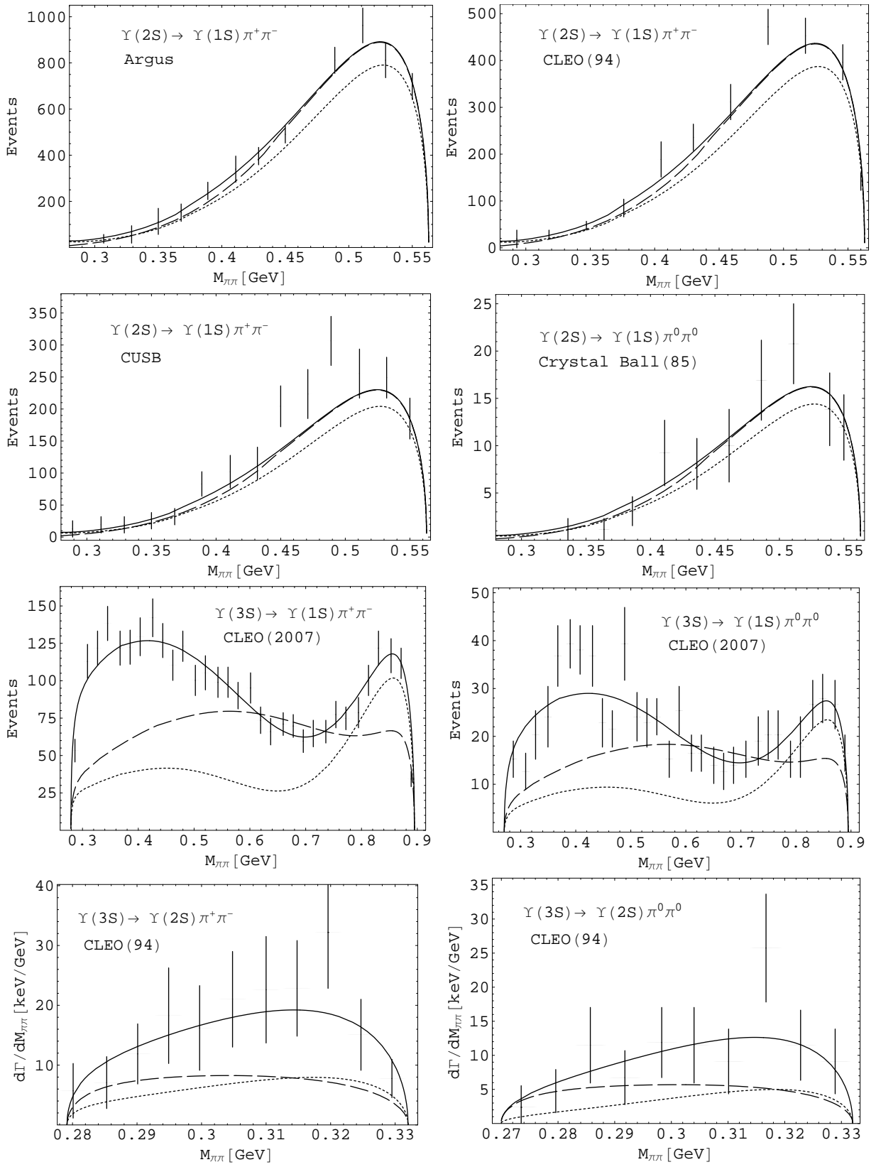
FIG. 2: The decays \Upsilon(2S) \rightarrow \Upsilon(1S)\pi\pi (two upper panels), \Upsilon(3S) \rightarrow \Upsilon(1S)\pi\pi (middle panel) and \Upsilon(3S) \rightarrow \Upsilon(2S)\pi\pi (lower panel). The solid lines correspond to contribution of all relevant f_0 -resonances; the dotted, of the f_0(500) , f_0(980) , and f'_0(1500) ; the dashed, of the f_0(980) and f'_0(1500) .
