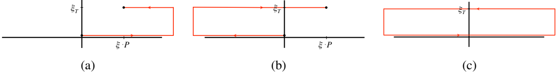
Figure 1: The so-called plus and minus staple-like gauge links (a) U_{[0,\xi]}^{[+]} and (b) U_{[0,\xi]}^{[-]} run along the light-front ( \xi \cdot n = 0 ) via plus or minus light cone infinity respectively, connecting the points 0 and \xi . The plus and minus gauge links make up the Wilson loop (c) U^{[\square]} \equiv U_{[0,\xi]}^{[+]} U_{[\xi,0]}^{[-]} = U_{[0,\xi]}^{[+]} U_{[0,\xi]}^{[-]\dagger} , with transverse extent \xi_T (the longitudinal extent is infinite).
