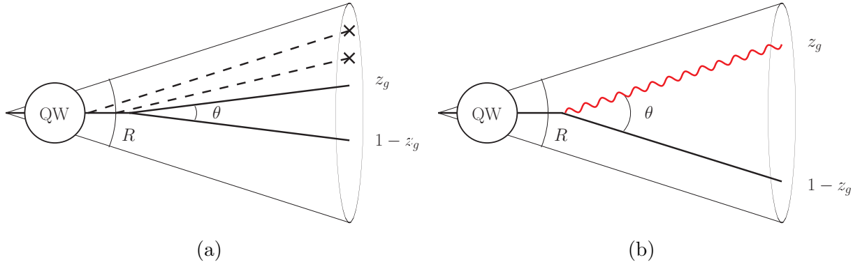
Figure 1: Coherent energy loss. The blob on the first propagator illustrates the coherent energy loss of the jet which does not affect the groomed jet structure. Its range extends however along the whole in-medium path length. (a) Vacuum radiation, including real, groomed emissions that are marked by a cross. (b) Hard, quasi-collinear medium-induced radiation (depicted by a red, wavy line) emitted inside the jet cone.
