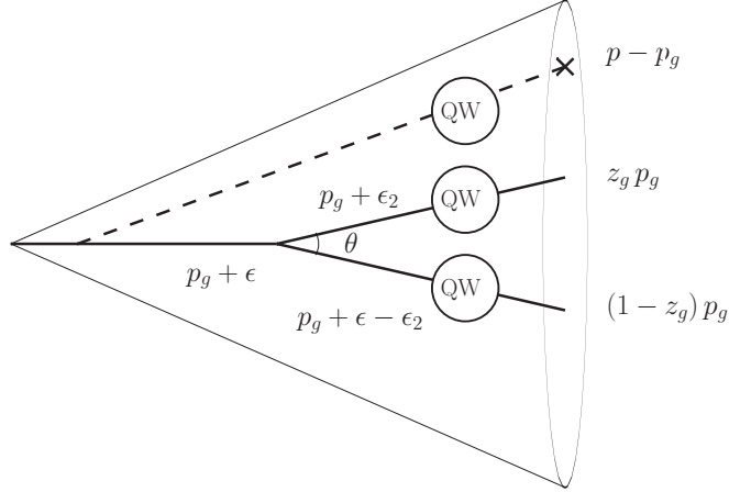
Figure A.4: Illustration of the splitting function in the incoherent approximation.
