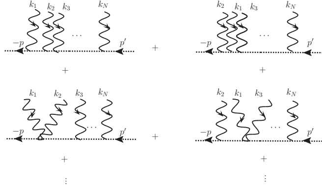
Figure 1: Multi-photon Compton-scattering diagram.
