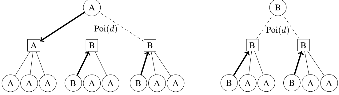
Figure 2: Illustration of the inclusion graph of the d -tree \mathbf{B}_d for d = 3 . Circles represent (d - 1) -faces, and squares are d -faces, each vertex is marked with the face's type. The thick arrows are included only to explain how the selection process of S_d(n, 1) is reflected in the d -tree. A dashed line demonstrate that the number of type ( B ) d -faces descending from a (d - 1) -face is \text{Poi}(d) randomly distributed. Since the root has type ( A ), the information in this figure completely determines the distribution of \mathbf{B}_d .
