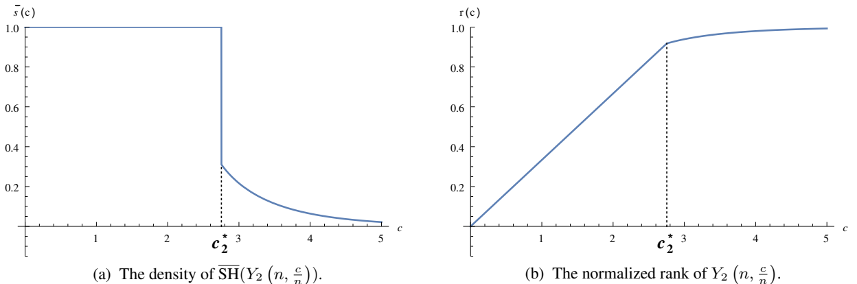
Figure 1: Plot of the functions \bar{s} and r for dimension d = 2 .
