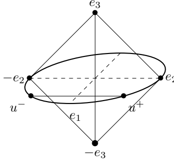
Figure 3: Phase space with the set \{W_3 = 0\} = \mathbb{S}^1 \cup \{\pm e_3\}
