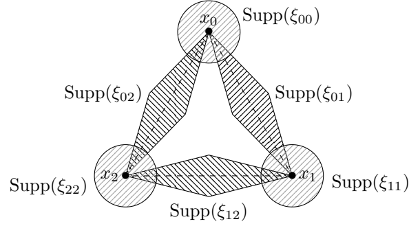
Figure 5: The supports of the \xi_{ij} when d = 2
