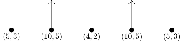
FIGURE 2. Resolution graph of y^5 + x^2 y^2 + x^5 with (N, \nu) -data.
