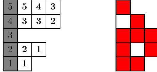
FIGURE 8. The semistandard key tableau equivalent to the filling T \in \mathfrak{DSSF}(a) of Example 4.29, together with its corresponding Kohnert diagram.
