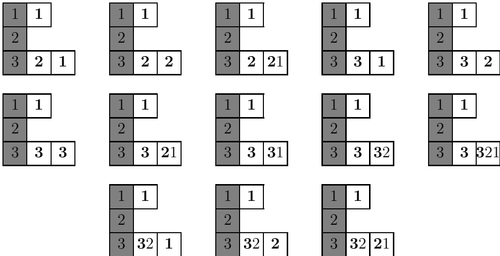
FIGURE 7. The 13 elements of \overline{\mathfrak{D}}\text{SSF}(102) .
