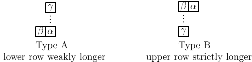
FIGURE 3. Triples for skyline diagrams.
