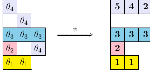
FIGURE 10. The threading of the Kohnert diagram K of Figure 8 and the corresponding filling \psi(K) \in \mathfrak{A}SSF(2, 1, 3, 0, 3) . Here, we have labeled the boxes of K by the threads of which they are part. The color-coding of the boxes of K is redundant with this labeling by threads, and the color-coding of the boxes of \psi(K) matches the color-coding of K .
