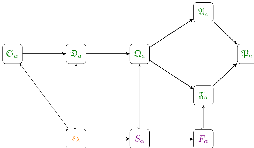
FIGURE 1. The nine cohomological families of polynomials considered here. Those depicted in orange are bases of \text{Sym}_n , those in purple are bases of \text{QSym}_n , and those in green are bases of \text{Poly}_n . The thinner hooked arrows denote that the basis at the tail is a subset of the basis at the head. The thicker arrows denote that the basis at the head refines the basis at the tail.
