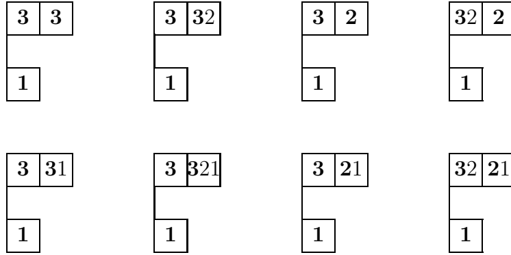
FIGURE 5. The eight elements of \overline{\mathfrak{A}}\text{SSF}(102) . The set \overline{\mathfrak{A}}\mathfrak{2}\overline{\mathfrak{P}}(102) consists of two fillings, specifically the leftmost filling in each of the two rows. Each of the eight illustrated fillings destandardizes to the leftmost filling in its row.
