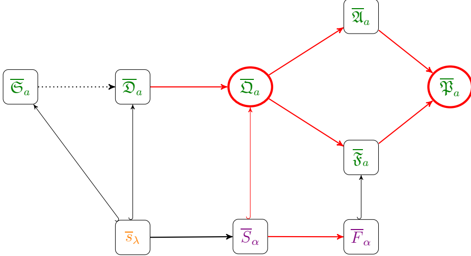
FIGURE 2. The K -theoretic analogues of the nine cohomological families of polynomials of Figure 1. As in Figure 1, families depicted in orange are bases of \text{Sym}_n , those in purple are bases of \text{QSym}_n , and those in green are bases of \text{Poly}_n . The thinner hooked arrows denote that the basis at the tail is a subset of the basis at the head. The thicker arrows denote that the basis at the head refines the basis at the tail. Those families and arrows that are original to this paper are marked in red. The dotted arrow is conjectural; see [RY15].
