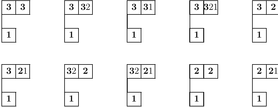
FIGURE 6. The ten elements of \overline{\Omega}\text{SSF}(102) .
