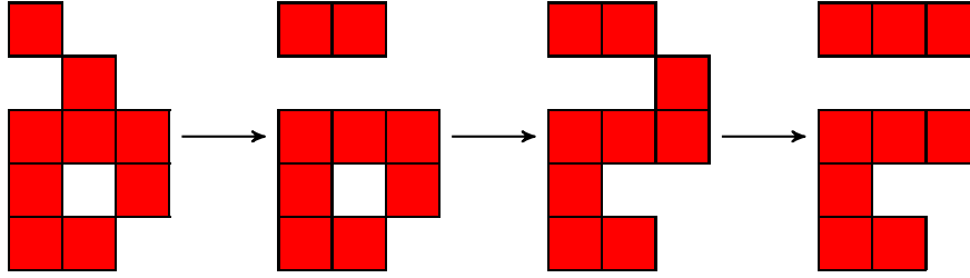
FIGURE 9. The iterative computation of the nearest skyline diagram of the Kohnert diagram from Figure 8.
