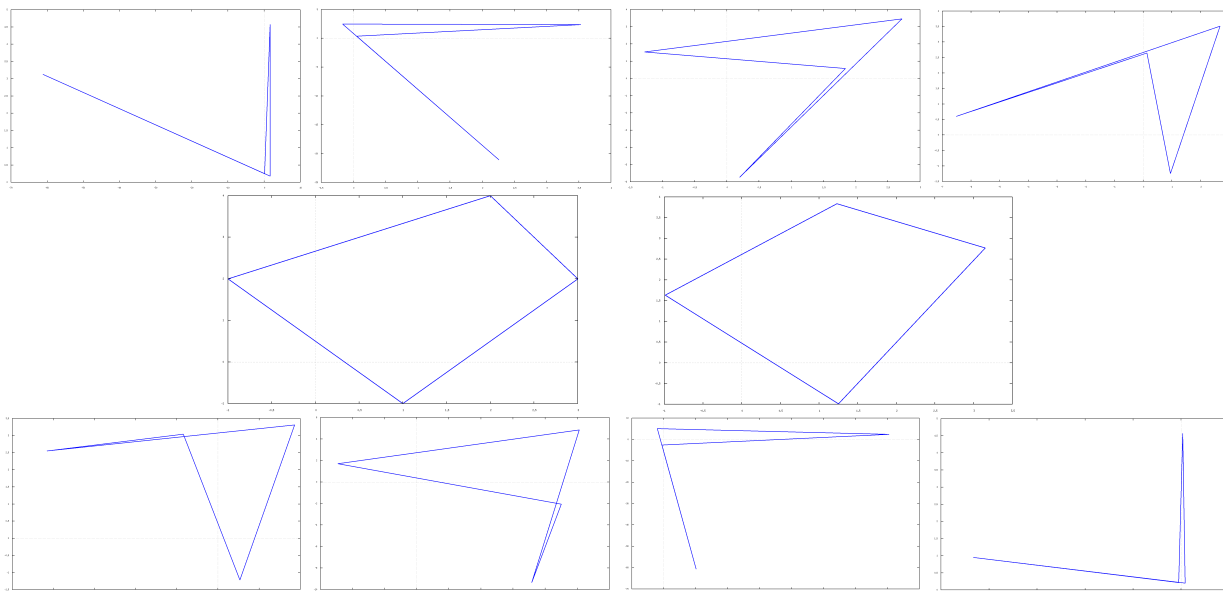
Figure 2: Ten real quadrilaterals having the same moments m_{ij} for i, j \in \{0, 1, 2\} .
