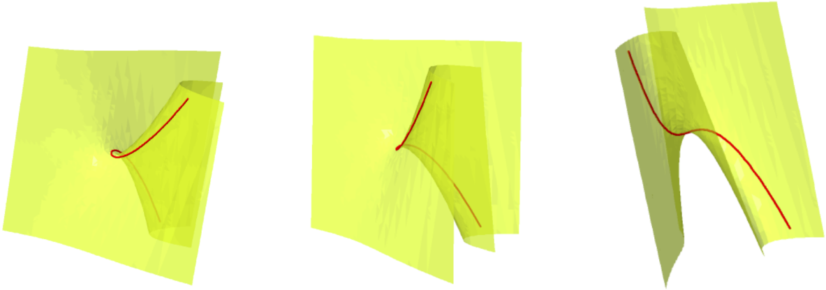
Figure 1: The cubic surface (4) represents the first three moments (2) of a line segment. Segments of length zero correspond to points on the twisted cubic curve (shown in red).
