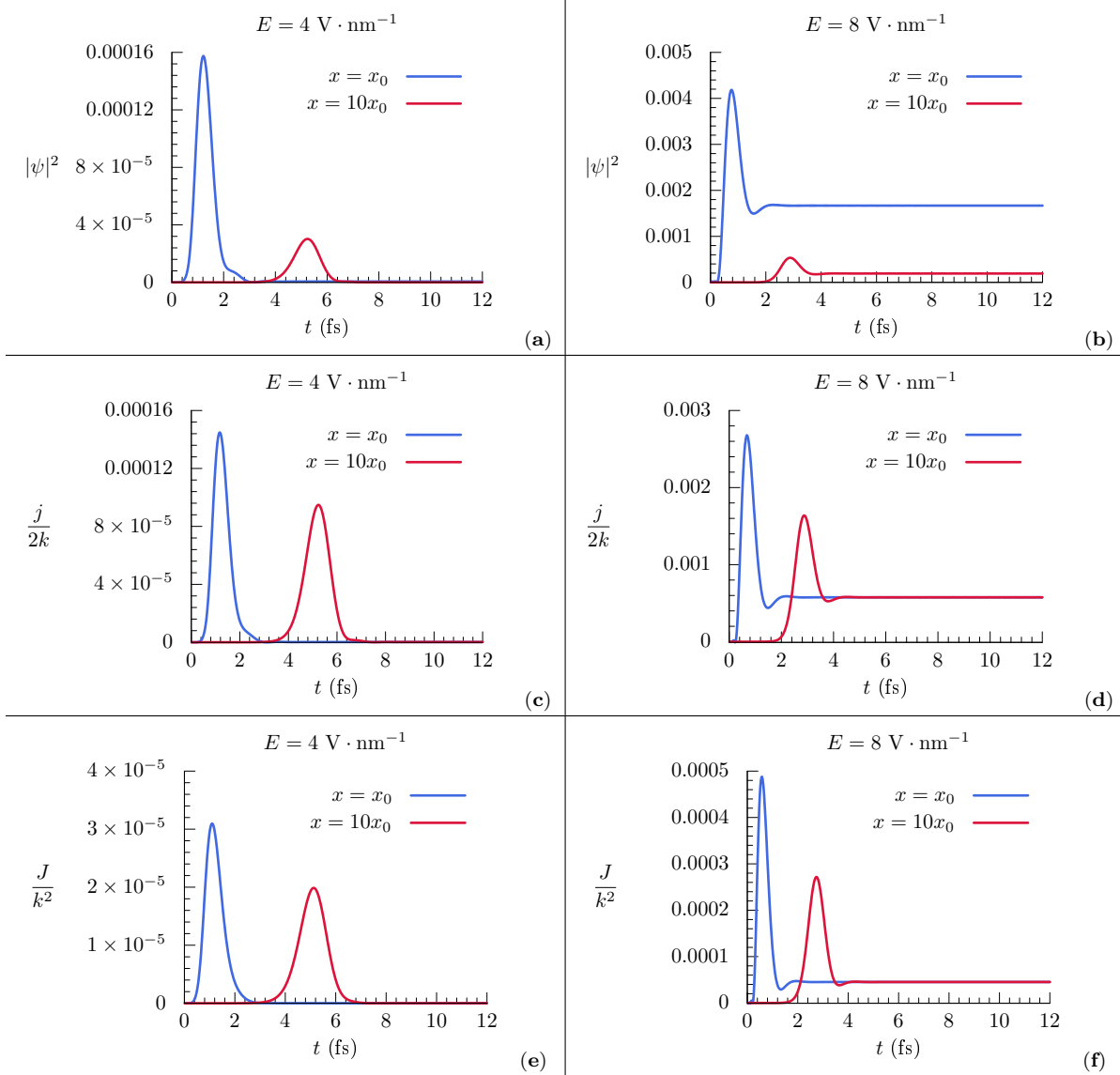
FIGURE 3. The density (a),(b), current (c),(d) and integrated current (e),(f) as a function of time at x = x_0 \equiv \frac{2U - k_F^2}{2E} and x = 10x_0 . We have taken U = 9 eV and k^2/2 = k_F^2/2 \equiv E_F = 4.5 eV. In (a),(c),(e), the field is E = 4 \text{ V} \cdot \text{nm}^{-1} and x_0 \approx 1.1 nm. In (b),(d),(f), E = 8 \text{ V} \cdot \text{nm}^{-1} and x_0 \approx 0.56 nm. In (a),(c),(e), the plots seem to indicate that the curves converge to 0, but they actually tend to small finite values.
