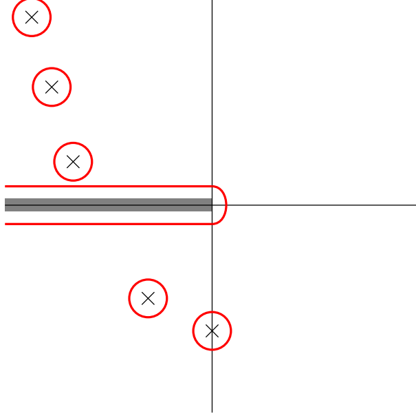
FIGURE 2. The deformed integration contour goes around the poles (one of which is on the imaginary axis, at -ik^2/2 , while the others are in the negative real half-plane) and goes along the branch cut on the real negative axis.
