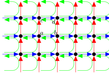
Figure 2: A finite fragment of the intended structure. The blue arrows represent the H-relations and the red ones the V-relations. The green curves represent the N-relations, e.g. Nabdc .
