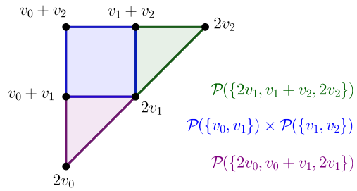
FIGURE 8. The space G_2 in Example 1.14
