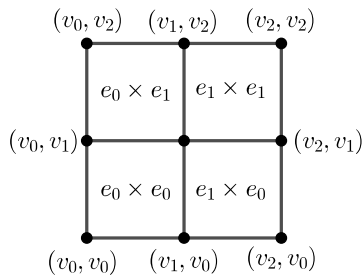
FIGURE 7. The space G^2 in Example 1.14
