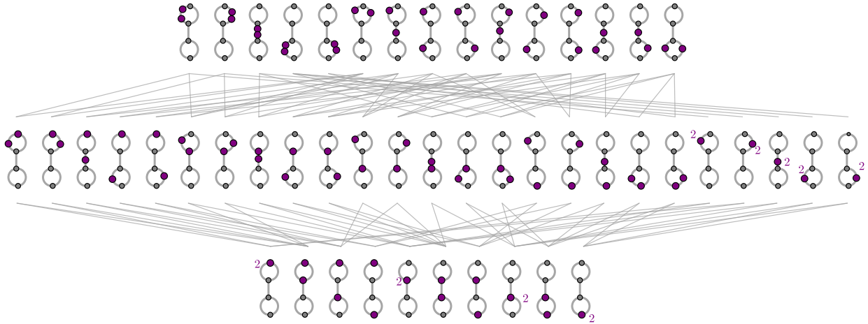
FIGURE 10. The poset \Xi_d(G) for the dumbbell graph G and d = 2 .
