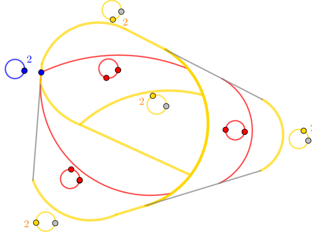
FIGURE 9. The second symmetric power (S^1)_2 , as in Example 1.15.
