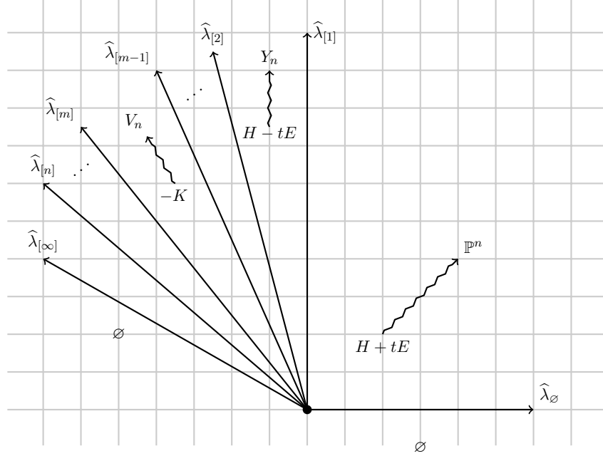
FIGURE 3. Portion of \Sigma_{\text{GKZ}} generated by E and H , and walls relating \mathbb{P}^n , Y_n , and V_n and their linearizations.
