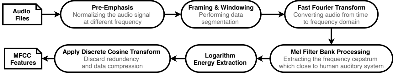
Figure 3: MFCC pipeline.
