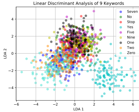
Figure 11: LDA of 9 keywords.
