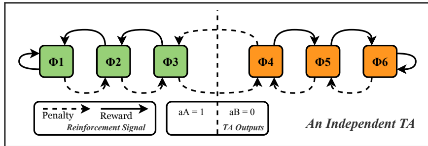
Figure 16: Mechanism of a TA.
