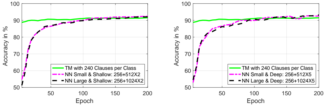
(a) Convergence of the TM against shallow NNs.
