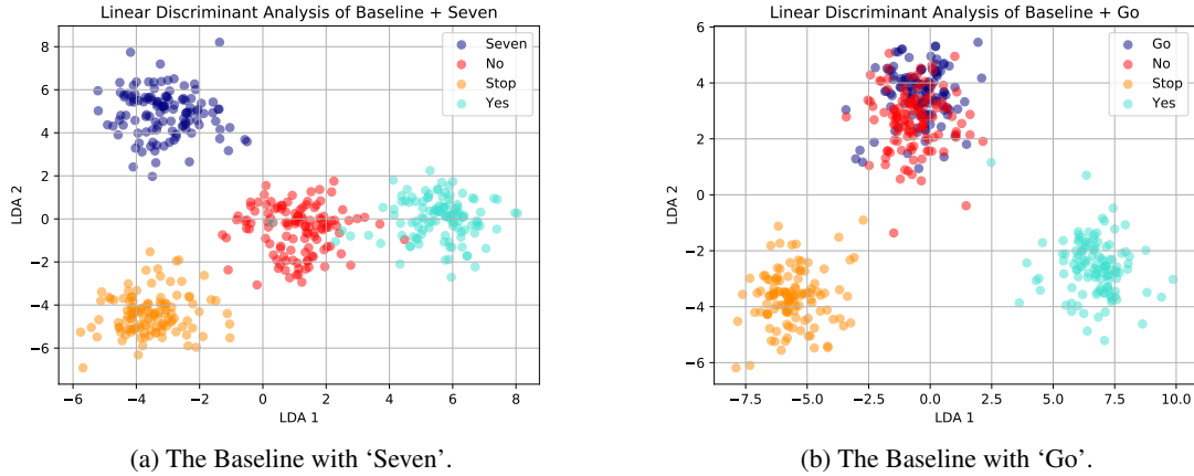
Figure 12: The LDA of 4 keywords - the Baseline with one other.
