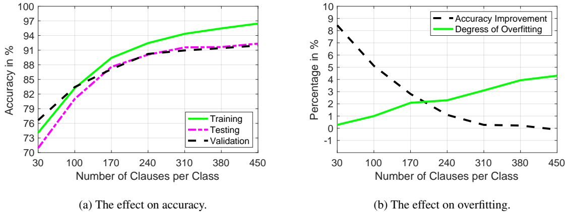
Figure 13: Effect of increasing the number of clauses on accuracy and overfitting.
