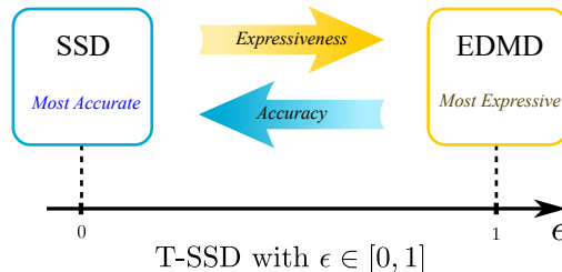
Figure 1. T-SSD generalizes SSD and EDMD. Given an arbitrary finite-dimensional function space, by changing the design parameter \epsilon \in [0, 1] in T-SSD, one can strike a balance between the invariance proximity of the identified subspace (i.e., the accuracy of the resulting model based on the available data) and its expressiveness.
