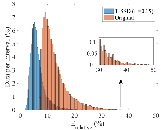
Figure 7. Relative linear prediction error on test data for the dictionary identified with T-SSD ( \epsilon = 0.15 ) and the original dictionary.
