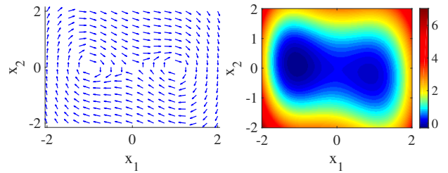
Figure 5. Vector field (left) and eigenfunction with eigenvalue \lambda = 0.9839 (right) for (43).
