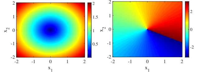
Figure 3. Absolute value (left) and phase (right) of the eigenfunction with eigenvalue \lambda = 0.9938 + 0.0195j for (40).
