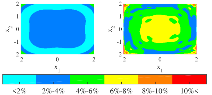
Figure 4. Relative linear prediction error for dictionary identified by T-SSD ( \epsilon = 0.05 ) (left) and the original dictionary (right) for (40).
