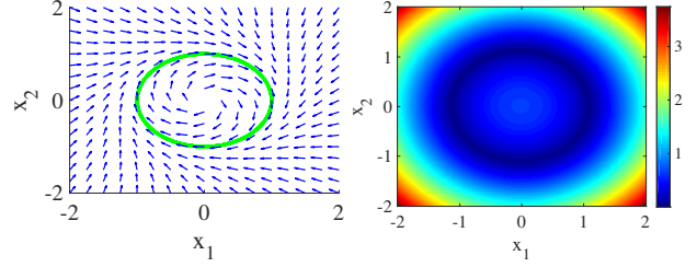
Figure 2. Vector field and periodic orbit of system (40) (left) and the absolute value of eigenfunction with eigenvalue \lambda = 0.9066 (right).
