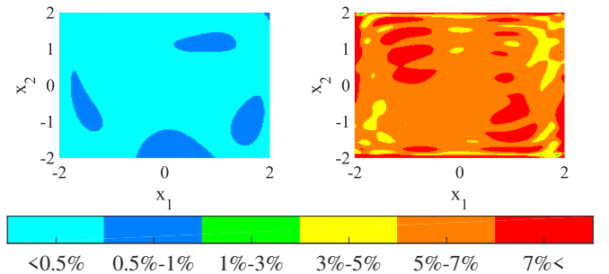
Figure 6. Relative linear prediction error for dictionary identified by T-SSD ( \epsilon = 0.02 ) (left) and the original dictionary (right) for (43).
