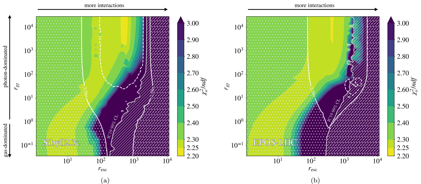
FIG. 5. Reduced \chi^2 of UHECR model predictions of the astrophysical neutrino flux as a function of model parameters r_{\text{esc}} \equiv \tau_{\text{esc}}^{\text{ref}}/\tau_{\text{int}}^{\text{ref}} and r_{g\gamma} \equiv \tau_g^{\text{ref}}/\tau_\gamma^{\text{ref}} for SIBYLL2.3C (left) and EPOS-LHC (right). Contours mark best-fitting region to CR data (dashed white contour) and 99% CL exclusion regions based on UHECR data (solid white contour and dotted region) and non-observation of neutrinos above 10^{15.9} eV (grey contour and hatched region).
