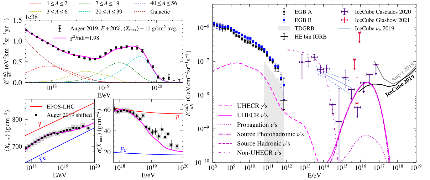
FIG. 6. Predictions of the UHECR source model producing the best description of the astrophysical neutrino flux for EPOS-LHC. Left: Same as in Fig. 1, except the red and blue solid lines show the \langle X_{\max} \rangle and \sigma(X_{\max}) predictions of EPOS-LHC for pure proton and iron models. Right: Same as in Fig. 1.
