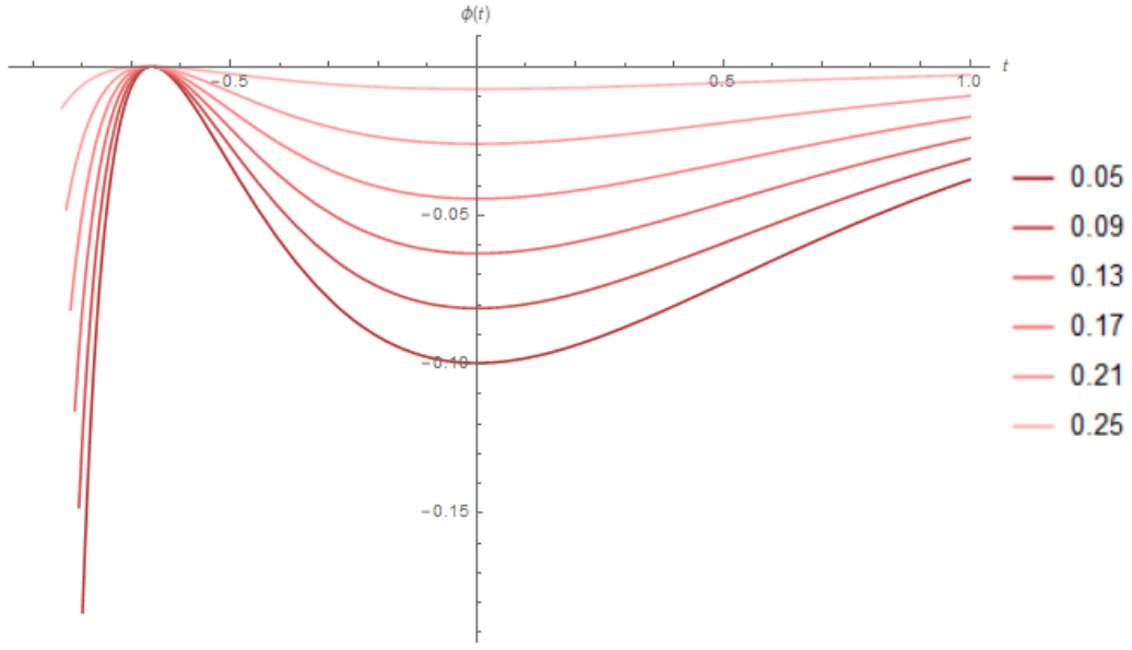
FIG. 3: Scalar field as a function of dimensionless cosmic time for \Omega_A = 1 , \sigma = 52 and \lambda = 10 . Different colors represent different amounts of 'true' matter content.
