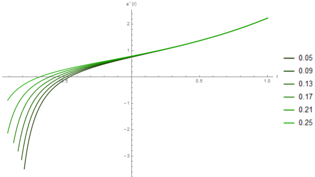
FIG. 2: Second derivative of the scale factor as a function of dimensionless cosmic time for \Omega_A = 1 , \sigma = 52 and \lambda = 10 . Different colors represent different amounts of 'true' matter content.
