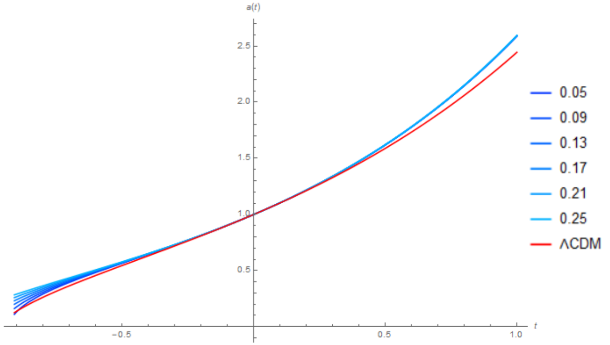
FIG. 1: Scale factor as a function of dimensionless cosmic time for \Omega_A = 1 , \sigma = 52 and \lambda = 10 . Different colors represent different amounts of 'true' matter content \Omega_{0,m} . The red curve represents \Lambda CDM model.
