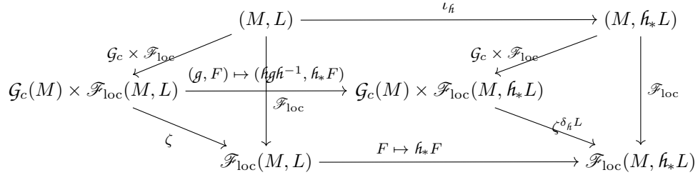
FIGURE 6. Behaviour of \zeta under the application of a symmetry \mathfrak{h} \in \mathcal{G}_c(M) and the induced change of the Lagrangian.
