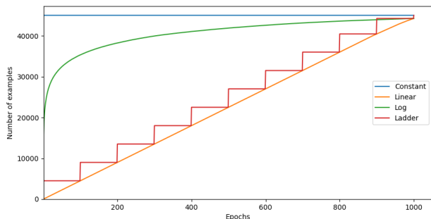
Fig. 6. Pacing functions: different increment functions can be chose to increase the variability of data in the training set. In this example, we have constant (conventional training), linear, logarithm, and ladder functions.
