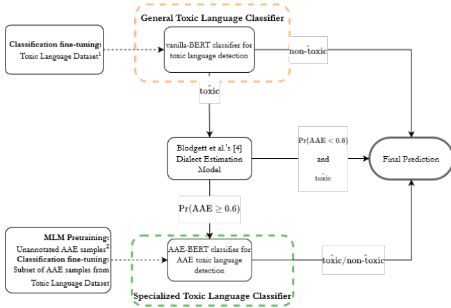
Fig. 1. The Hierarchical Ensemble (HxEnsemble) Framework 1 Training set of DWMW17, FDCL18, Toxic, or Hate is used. More details about these datasets can be found in Table 1. 2 The unannotated AAE samples used for the MLM pre-training come from Blodgett et al. [4]
