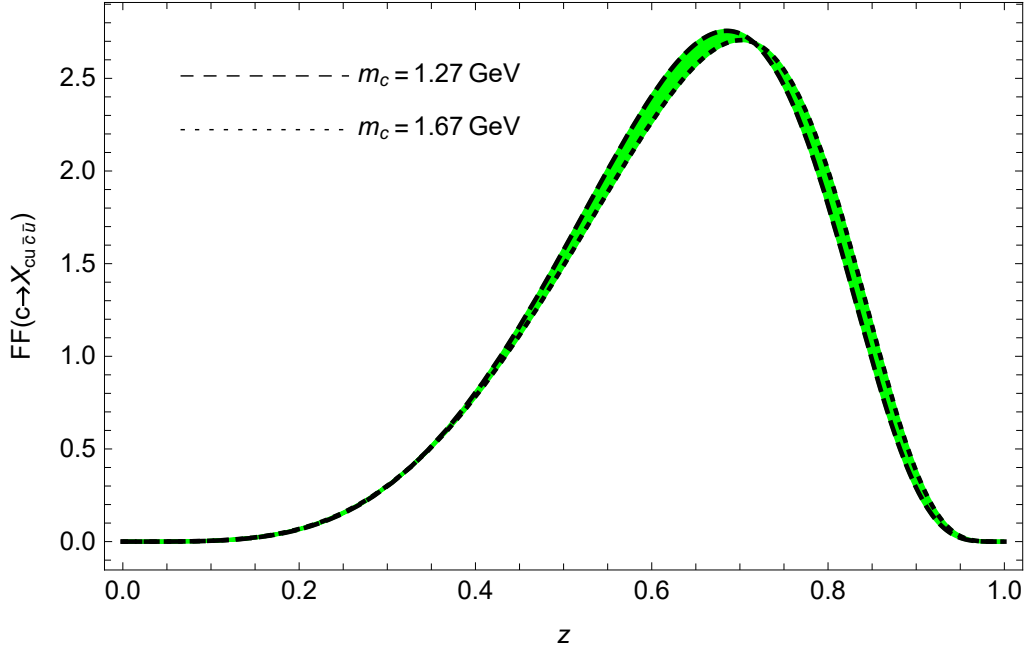
Figure 2: Fragmentation of c -quark into heavy tetraquark X_{cu\bar{c}\bar{u}} at lowest-order of perturbative QCD. The uncertainty band due to the variation of charm mass is also shown.
