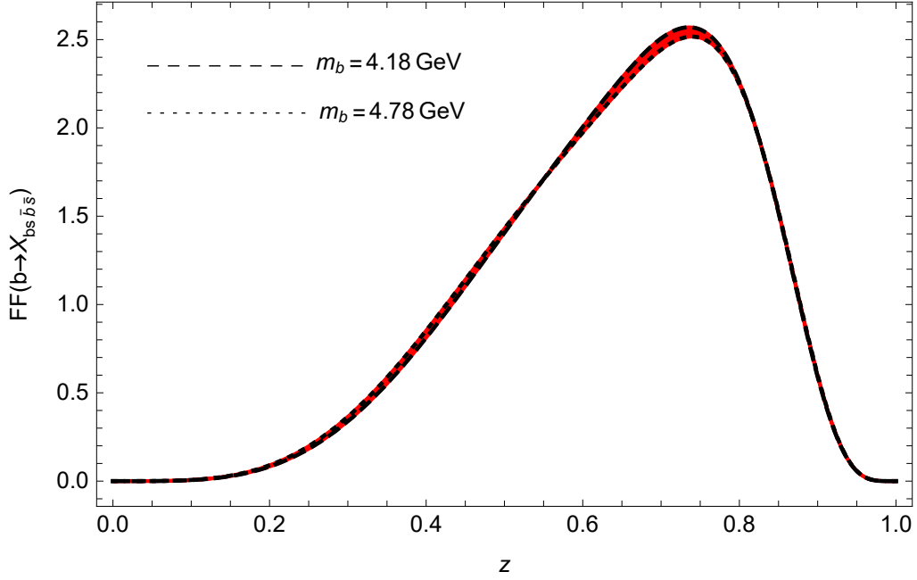
Figure 3: The b \rightarrow X_{bs\bar{s}} FF at leading order perturbative QCD along with the uncertainty band of bottom mass.
