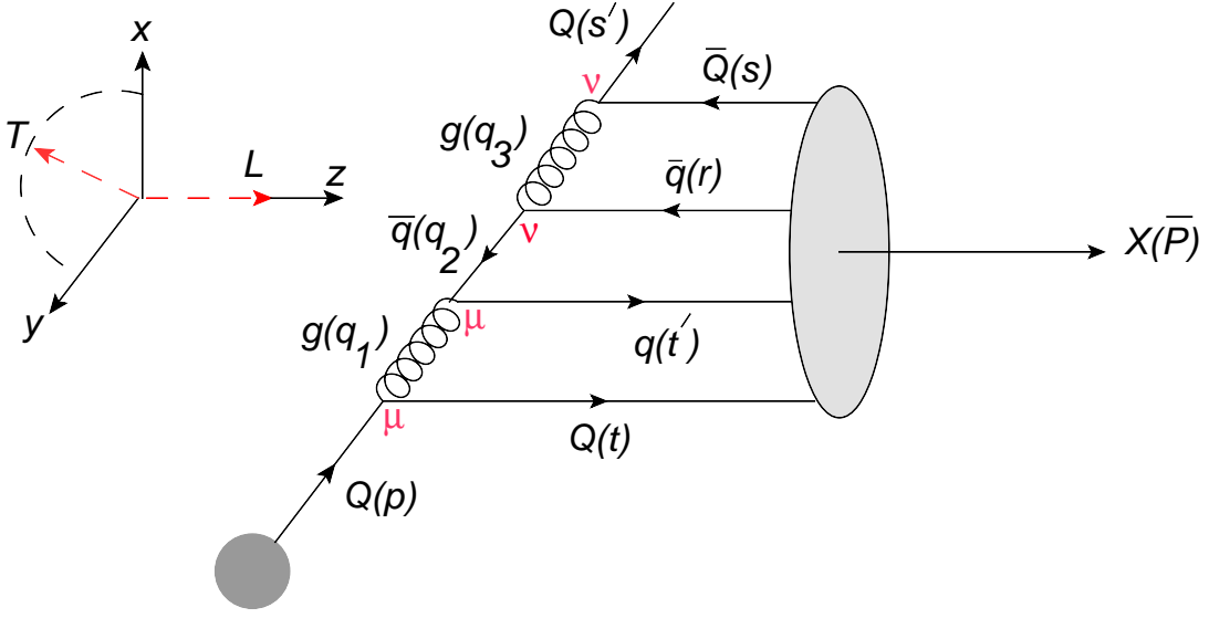
Figure 1: The lowest order Feynman diagram contributing to the fragmentation of a heavy quark Q into a heavy tetraquark X(Qq\bar{Q}\bar{q}) . The four momenta are also labeled.
