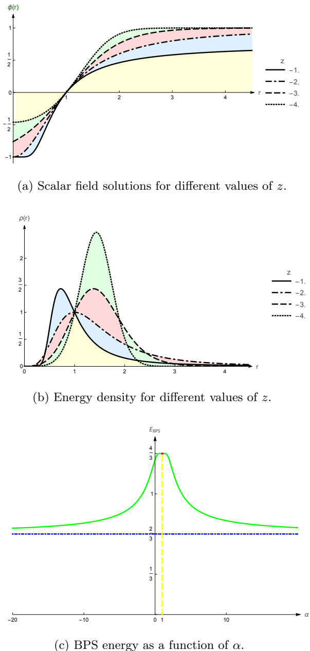
FIG. 1. Spatially-localized profile of the scalar field (a) and the energy density (b) for D = 3 + 1 and different values of the dynamical exponent z , where we can observe the behavior of the solution for \alpha > 1 ( z = -1 ), \alpha = 1 ( z = -2 ) and \alpha < 1 ( z = -3 and z = -4 ). The BPS energy as a function of \alpha is depicted in (c).
