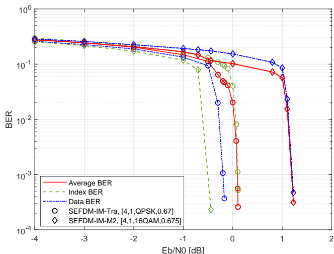
Fig. 14. Error performance of SEFDM-IM systems with different modulation schemes.
