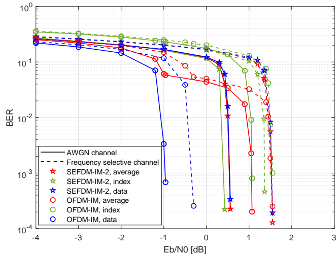
Fig. 11. Error performance of the coded SEFDM-IM-2 system at 1.1 bit/s/Hz and the OFDM-IM system at 1 bit/s/Hz with and without frequency selective channel.
