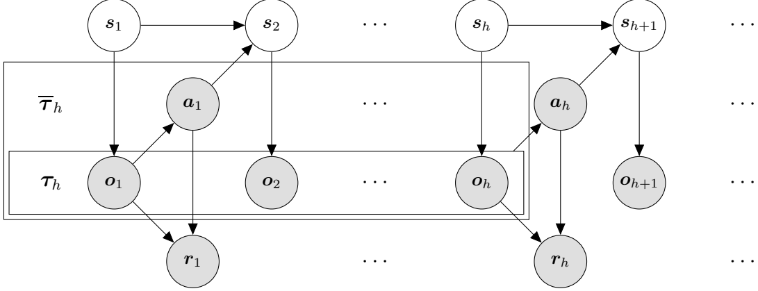
Figure 1: Directed acyclic graph of a POMDP. Here, we denote by \tau_h = (\mathbf{o}_1, \dots, \mathbf{o}_h) the observation history and \bar{\tau}_h = (\mathbf{o}_1, \mathbf{a}_1, \dots, \mathbf{o}_{h-1}, \mathbf{a}_{h-1}, \mathbf{o}_h) the full history. See Section 2.1 for more details.
