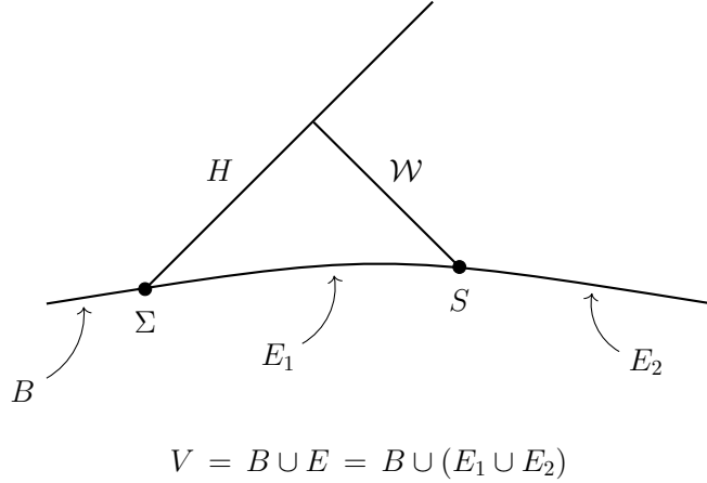
Figure 1: The set up for this section. The black hole horizon is represented by H = \partial I^+(B) \setminus \text{int}_V B .
