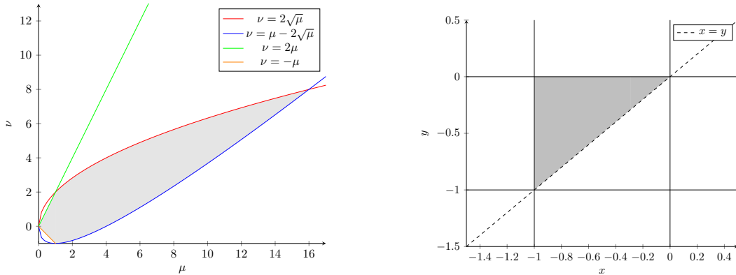
(a) Admissible (\mu, \nu) parameters (shaded).
