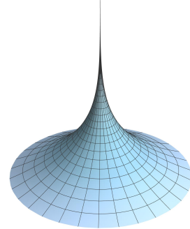
Figure 10: Naked Singularity, not infinitely long.
