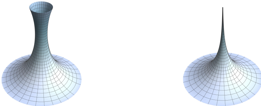
Figure 9: Stages of cusp formation. The cusp on the right is infinitely long.
