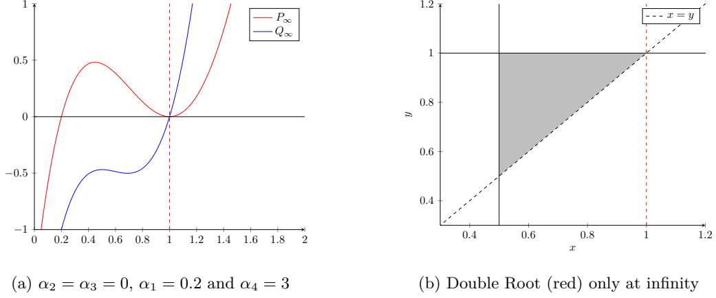
Figure 4: Example polynomials and region for metric with naked singularity at infinity.
