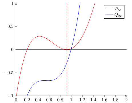
Figure 7: Cusp to Naked Singularity
