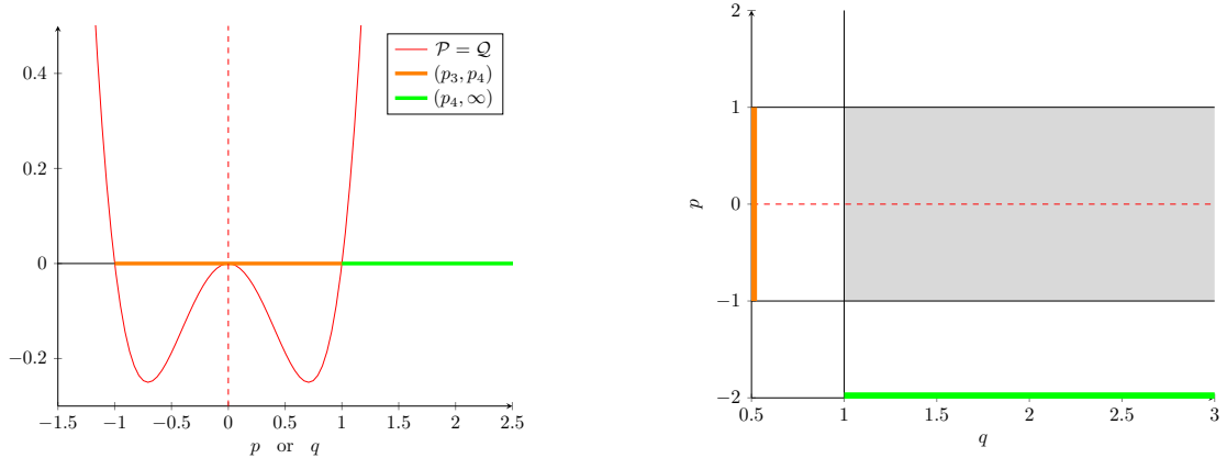
(a) Example of double root in \mathcal{P} with N = M . Intervals where \mathcal{P} and \mathcal{Q} are defined are highlighted.
