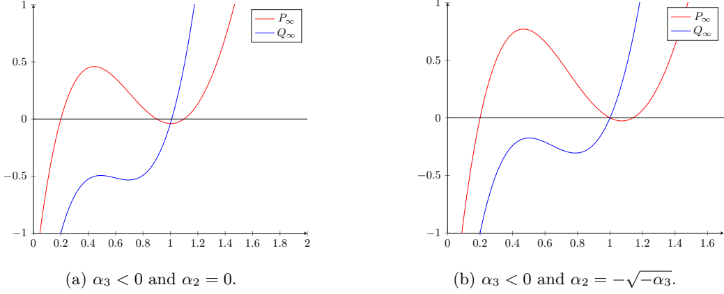
Figure 6: Conical Singularity to Naked Singularity
