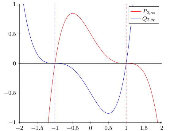
Figure 8: Two cusps at conformal infinity only .
