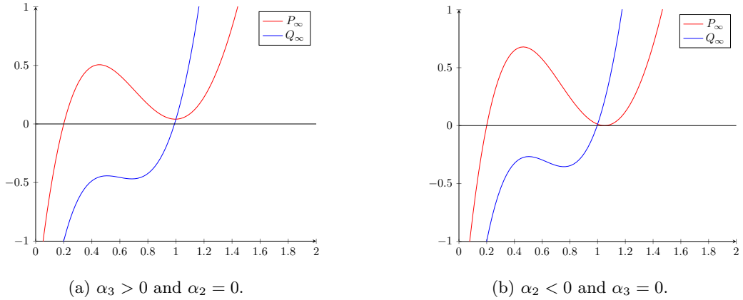
Figure 5: Smooth Metric to Naked Singularity
