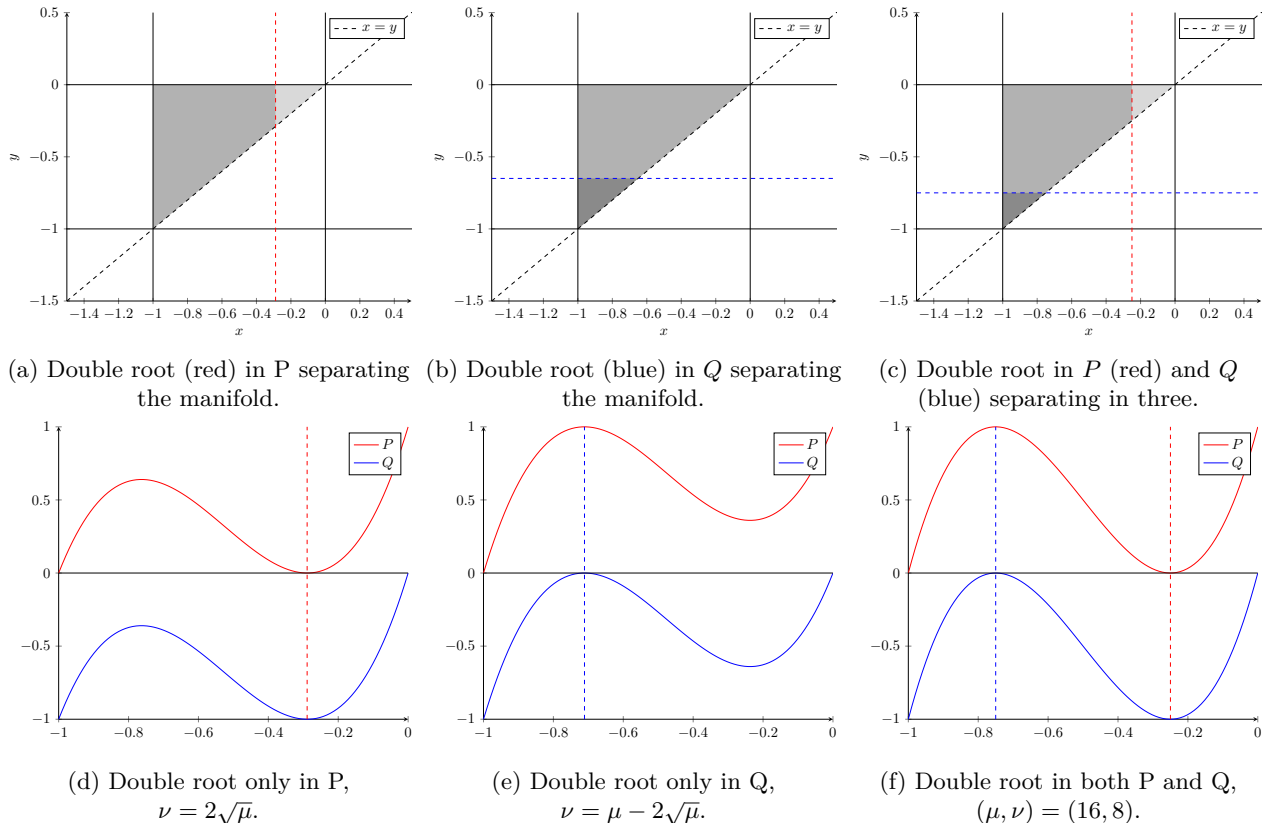
Figure 2: Different configurations of double roots.
