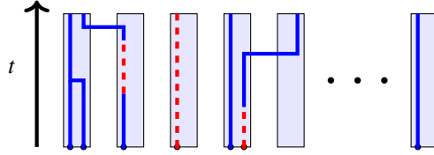
Figure 4: Picture of the evolution of lineages in the spatial coalescent. The purple blocks depict the colonies, the blue lines the active lineages, and the red dashed lines the dormant lineages. Blue lineages can migrate and become dormant, (i.e., become red dashed lineages). Two blue lineages can coalesce when they are at the same colony. Red dashed dormant lineages first have to become active (blue) before they can coalesce with other blue and active lineages or migrate. Note that the dual runs backwards in time . The collection of all lineages determines the genealogy of the system.
