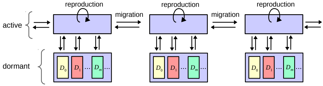
Figure 3: The spatial evolution in Model 2. Each colony has its own seed-bank. Resampling occurs within the active population in each colony. Migration occurs between active populations in different colonies (top layer). Exchange between the active and the dormant population occurs in each colony (transitions between the top layer and the bottom layer).
