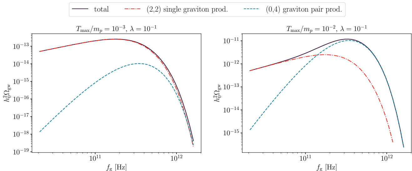
FIG. 6: Gravitational wave spectrum with respect to the present day GW frequency. The single graviton production processes which are of order \mathcal{O}(\lambda^2\kappa^2) = (2, 2) are shown as a red dot-dashed line. The graviton pair production processes are shown as a dashed blue line and are of order \mathcal{O}(\kappa^4) = (0, 4) . The total GW spectrum is shown as a solid black line. On the left we show a scenario where the maximum temperature is limited to 10^{-3} m_p . In the right figure we set the maximum temperature to T_{\max} = 10^{-2} m_p . In this case the graviton pair production processes yield an even larger contribution compared to the single graviton production processes. The GW spectra are calculated for a complex scalar model with g_*(T_{\max}) = 2 .
