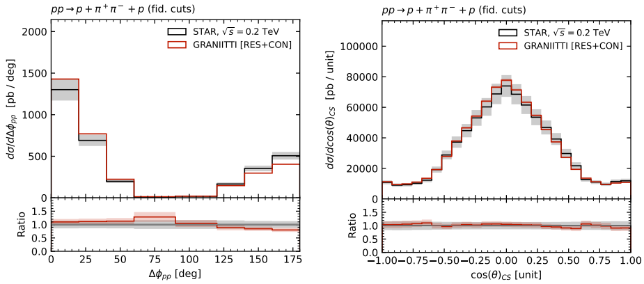
Fig. 5. Forward proton \Delta\phi_{pp} (left) and CS-frame angle \cos(\theta) of \pi^+ (right).
