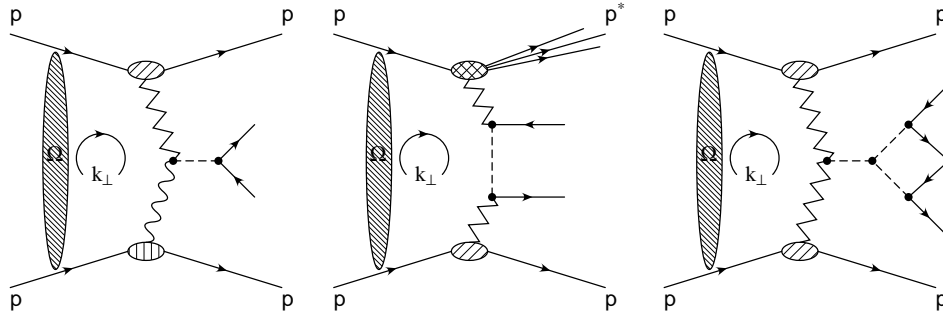
Fig. 1. Pomeron-Gamma-Resonance, Pomeron-Pomeron \rightarrow central hadron pair + one excited forward proton p^* and Pomeron-Pomeron-Resonance to a four-body central state. k_T is the screening loop 2D -momentum. For details, see [1].
