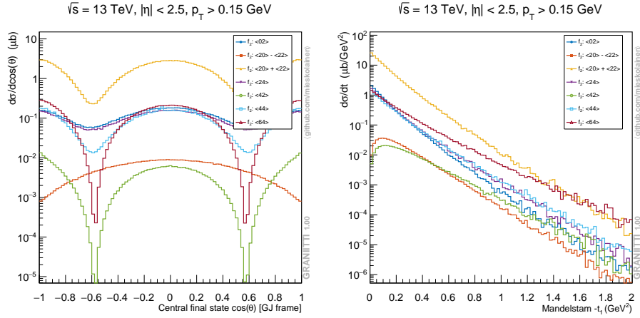
Fig. 3. Tensor Pomeron: Angular distribution \cos(\theta) of \pi^+ in the Gottfried-Jackson frame (left) and Mandelstam -t_1 for 7 spin-2 couplings (right). For details, see [1].
