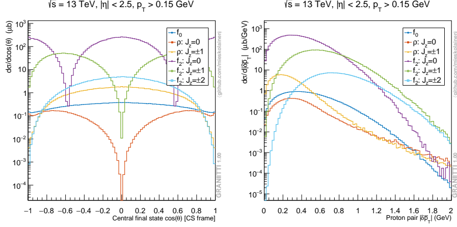
Fig. 2. Minimal Pomeron: Angular distribution \cos(\theta) of \pi^+ in the Collins-Soper frame for different diagonal spin polarization components (left). Forward proton p_T -vector difference (right). For details, see [1].
