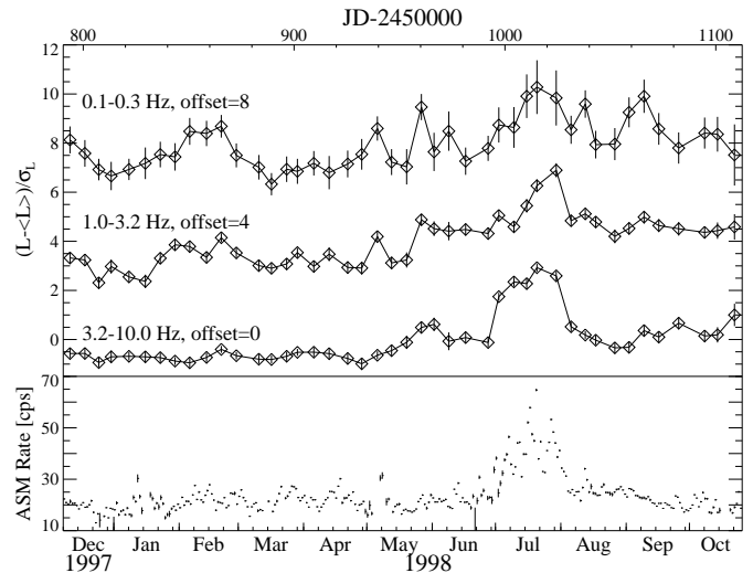
Fig. 2. Diamonds: Temporal evolution of the average lag between \lesssim 4 keV and 18.3–72.9 keV for the indicated frequency intervals. The deviation of the lag from its mean value as determined from all observations of 1998 for the respective frequency band, in units of its standard deviation is shown. Dashes: RXTE ASM 2–10 keV count rate binned to a resolution of 1 d.
