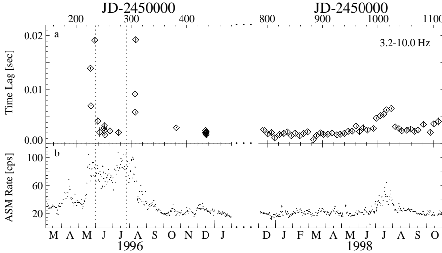
Fig. 3. a Temporal evolution of the absolute value of the average lag between \lesssim 4 keV and \sim 8-13 keV in the 3.2 to 10 Hz band and b ASM count rate for 1996 and 1998. The dotted lines denote the 1996 soft state.
