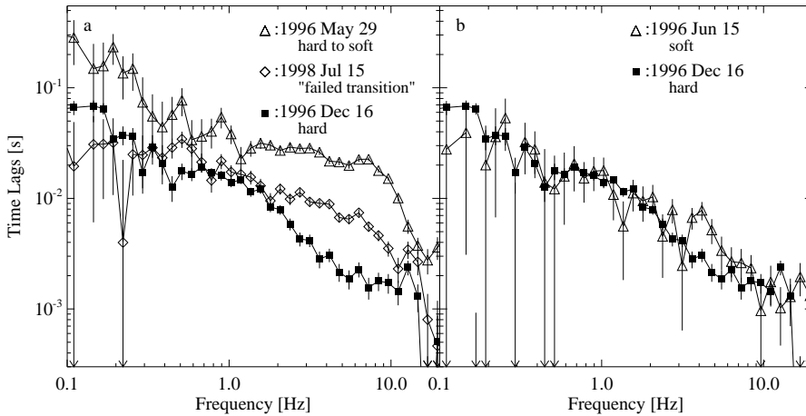
Fig. 4. X-ray lag spectra between \lesssim 4 keV and \sim 8 –13 keV. a Comparison of the hard to soft state transition, the 1998 July transitional state, and the typical hard state. b Comparison of the 1996 soft state and the hard state.
