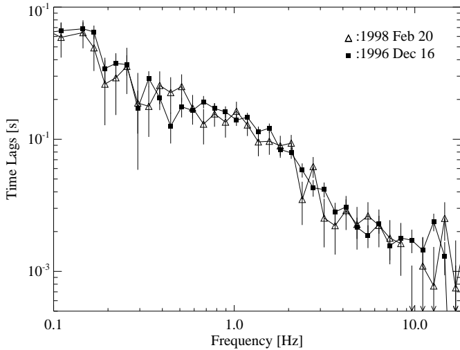
Fig. 1. Comparison of the X-ray lag spectrum for one of the 3 ks monitoring observations of 1998 with that obtained for \sim 30 ks of the RXTE observation of 1996 December 16. The lags have been measured between \lesssim 4 keV and \sim 8 –13 keV. Both examples are typical hard state observations.
