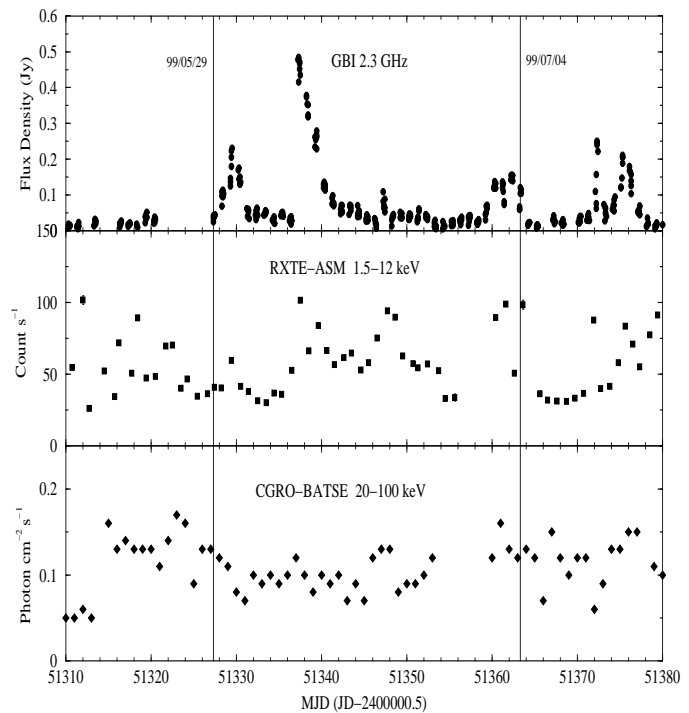
Fig. 3. Top. The radio behavior of GRS 1915+105 during our observations as recorded by the daily GBI monitoring. The vertical lines indicate the precise dates when the VLT-ISAAC spectra were obtained. Middle. The same kind of plot but showing the soft X-ray light curve of GRS 1915+105 from the RXTE-ASM data. Bottom. Another similar plot with the hard X-ray light curve of GRS 1915+105 from the CGRO-BATSE Earth occultation monitoring.
