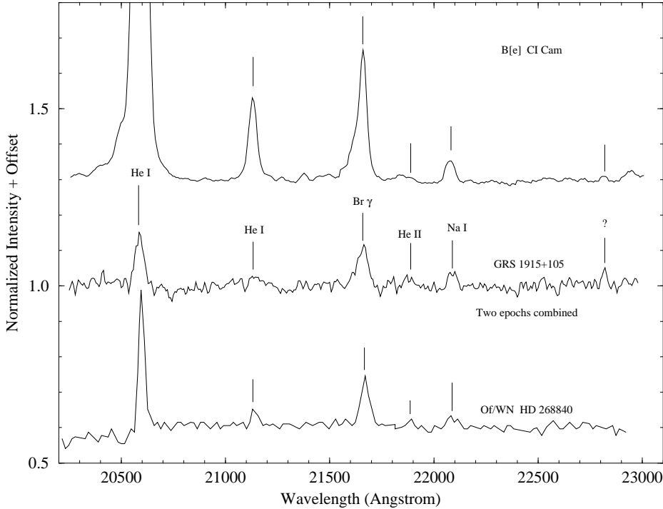
Fig. 2. Combined VLT spectrum of GRS 1915+105 (middle) obtained by averaging the data of the two epochs to increase signal-to-noise ratio in order to better detect any weak persistent features. The He II line in GRS 1915+105 appears barely visible because it is not present in the second epoch, while the faint He I feature may have some contribution from N III. The two comparison spectra are those of the B[e] system CI Cam (top) and the Ofpe/WN9 star HD 268840 (bottom) adapted from Clark et al. (1999) and Morris et al. (1996), respectively. The common features are identified on all plots and labeled for GRS 1915+105.
