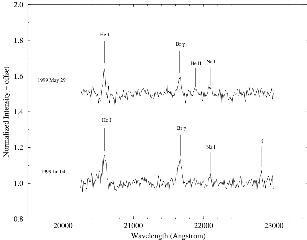
Fig. 1. VLT low resolution spectra of GRS 1915+105 obtained on 1999 May 29 (before a radio outburst) and 1999 July 04 (during a radio outburst) using the SK filter with ISAAC. The emission line identifications are indicated.
