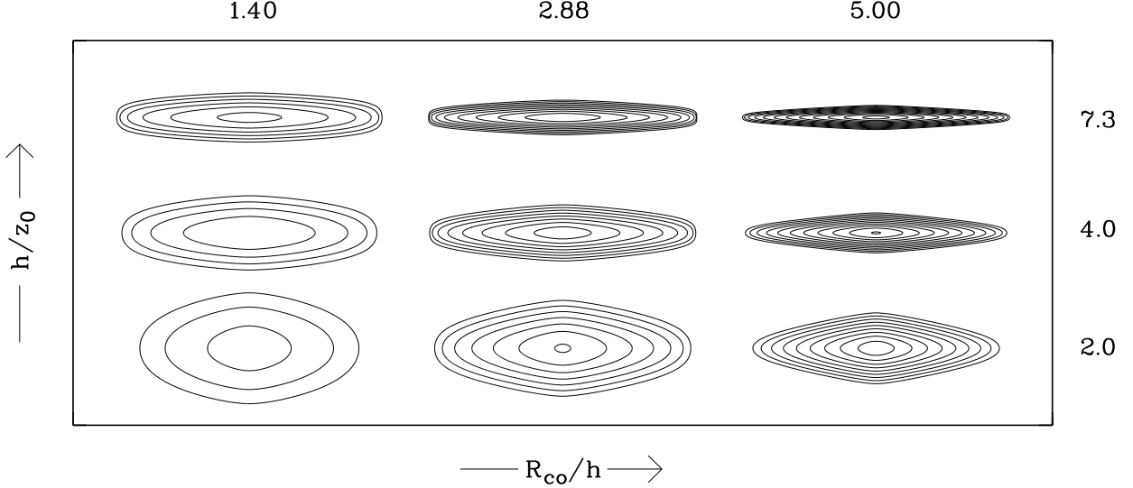
Fig. 1. Different galaxy models computed according to equation (4) with constant values for the ratio \frac{R_{\text{co}}}{h} within the columns, or \frac{h}{z_0} within the rows, whereas \hat{L}_{\text{tot}} and R_{\text{co}} are constant for all models using an isothermal description for the exact edge-on case
