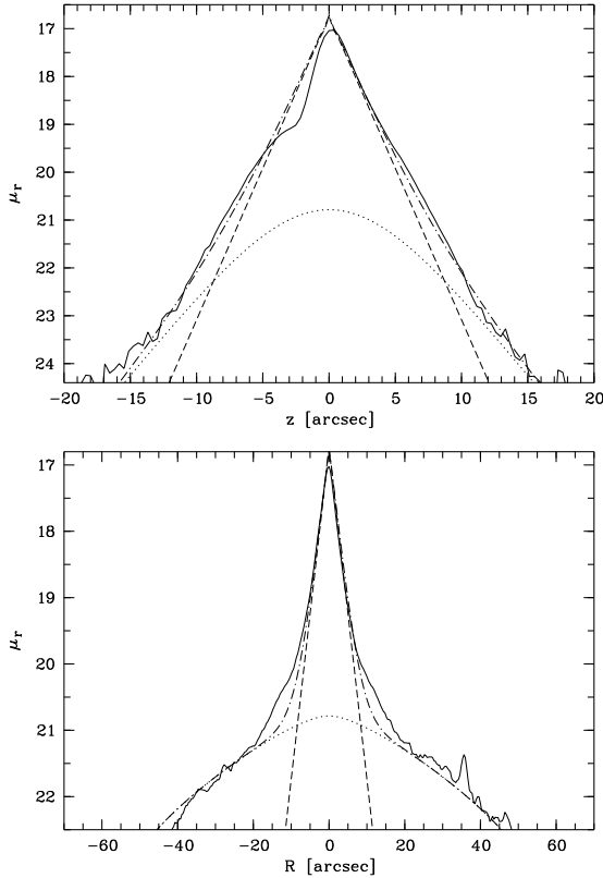
Fig. 3. Minor and major axes profile for ESO575059r15E2 (solid lines) together with the best disk model (dotted), the best bulge model (dashed), and the resulting combined profile (dotted-dashed).
