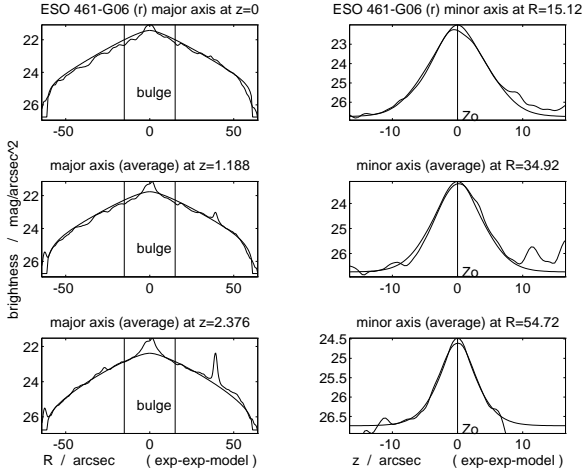
Fig. 2. Example of the fitting procedure: Set of typical radial (left panel) and vertical (right panel) profiles used for the fitting process of the galaxy ESO 461-006 together with the model.
