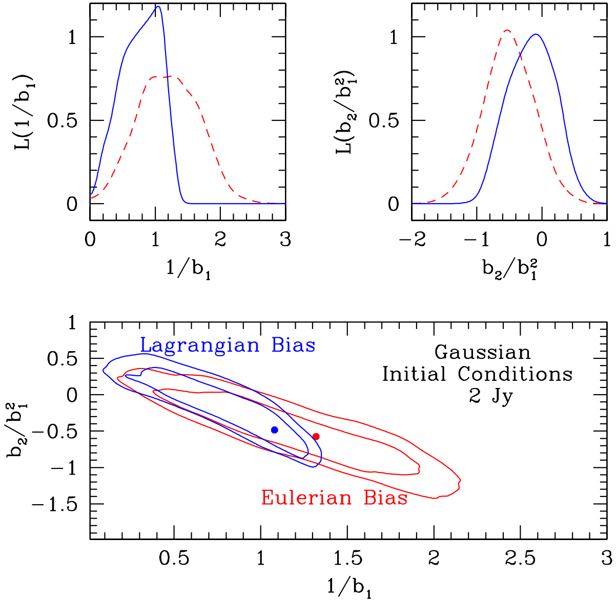
Fig. 11.— Likelihood analysis for the Lagrangian local bias model in the 2 Jy survey. Upper panels show marginalized likelihoods for Eulerian (dashed) and Lagrangian (solid) bias.
