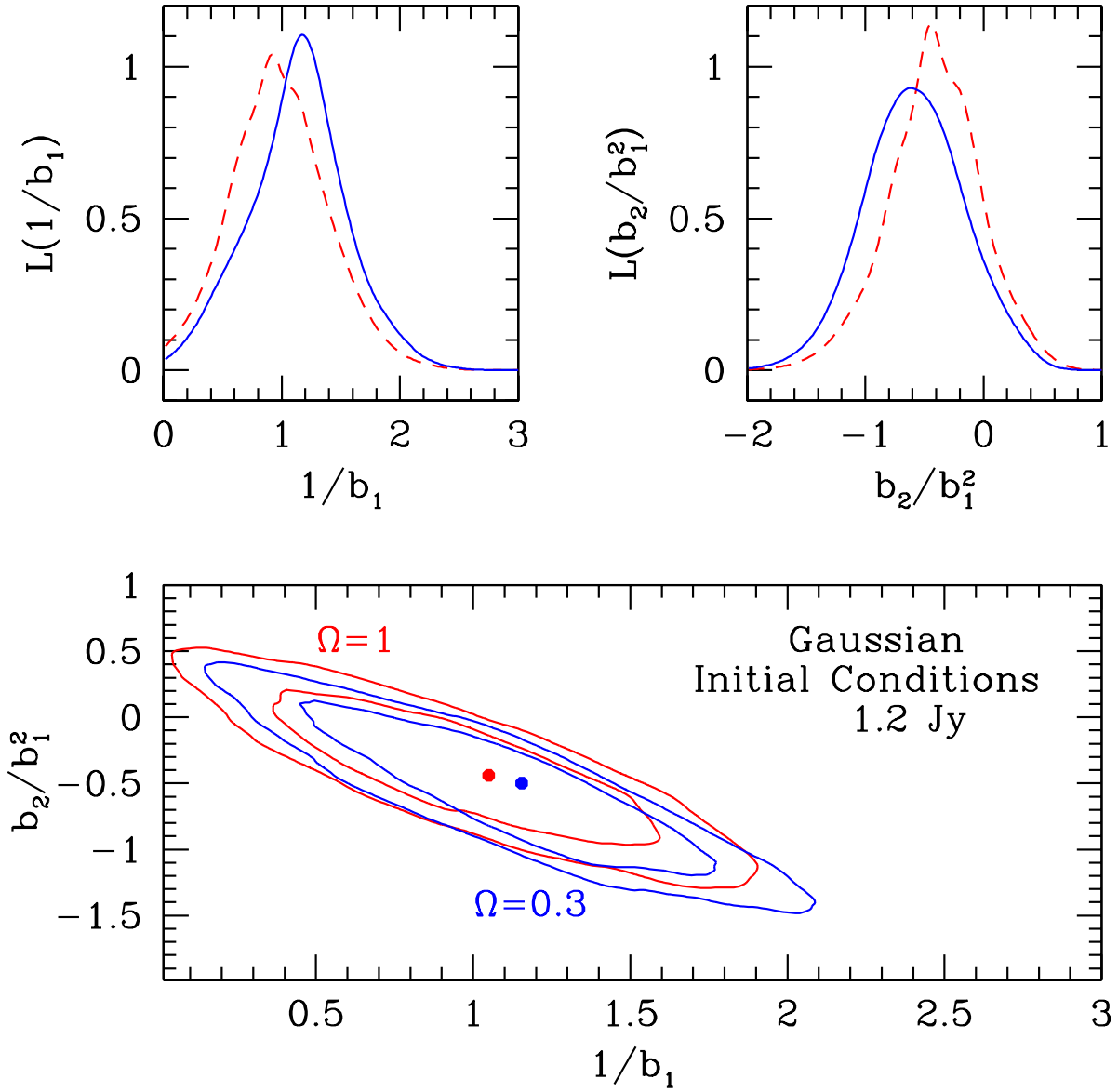
Fig. 9.— Same as Fig. 8, but showing the dependence of the results on \Omega_m in the 1.2 Jy catalog. In the upper panels, we show the marginalized likelihoods for \Omega_m = 1 (dashed) and \Omega_m = 0.3 (solid).
