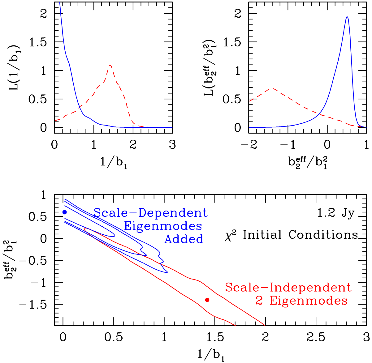
Fig. 10.— Likelihood analysis for \chi^2 initial conditions in the 1.2 Jy survey. Contours for the 2 highest S/N eigenmodes are 68%; contours for all eigenmodes are 68%, 90%, and 95%. Upper panels show marginalized likelihoods for 2 highest (dashed) and all (solid) eigenmodes.
