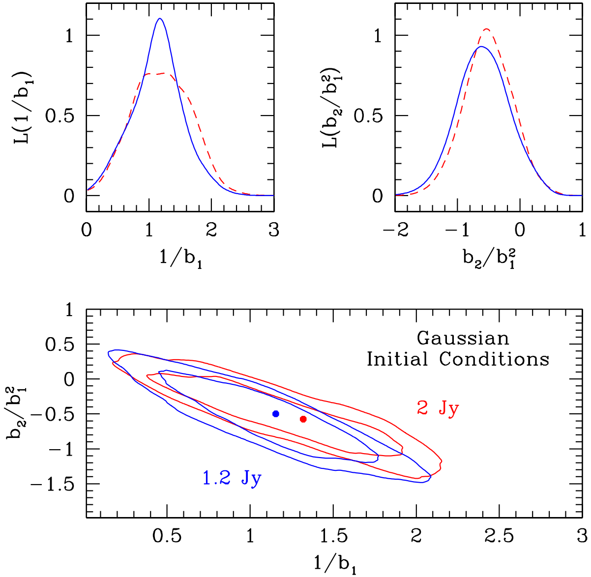
Fig. 8.— The bottom panel shows 68% and 90% likelihood contours for bias parameters assuming Gaussian initial conditions and \Omega_m = 0.3 for the 2 Jy and 1.2 Jy surveys. In the upper panels we show the marginalized likelihoods (normalization arbitrary) for 2 Jy (dashed) and 1.2 Jy (solid) catalogs.
