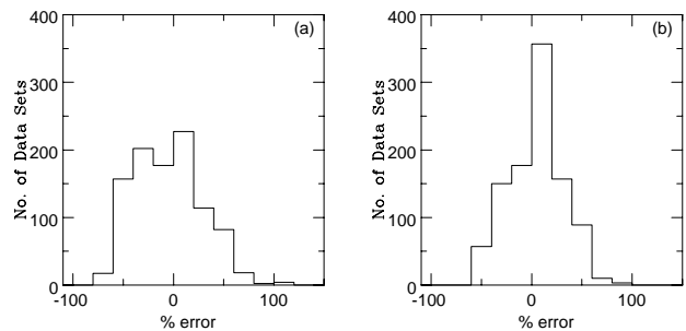
Figure 8 (a) Histogram showing the spread in mass estimates based on satellite datasets containing 10 objects at radii 20 \text{ kpc} < r < 500 \text{ kpc} whose proper motions have been measured using SIM and GAIA. The histogram shows the number of datasets out of 1000 which yielded a given percentage error in the total mass M . (b) As in (a), but for datasets of 20 satellites.
