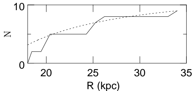
Figure 2. Cumulative number plot for the satellite galaxies. Also shown is a dotted curve representing the distribution from the assumed model, namely eq. (12) with a_s = 250 kpc.
