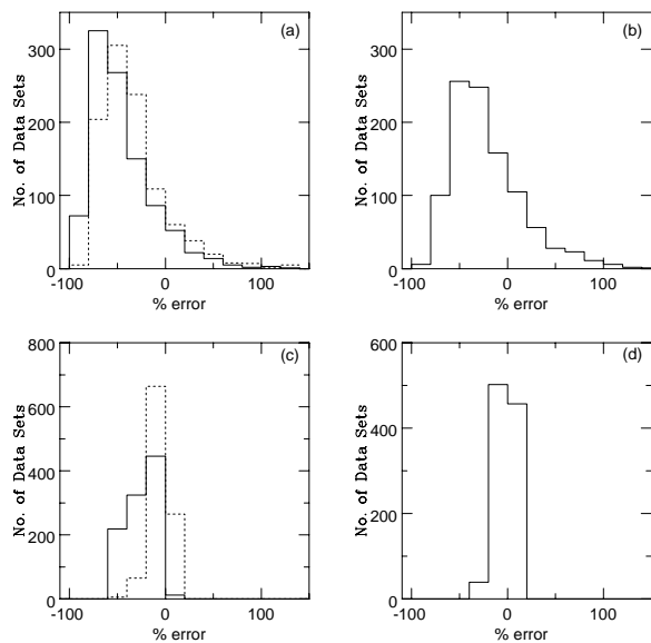
Figure 7 (a) Histogram showing the spread in mass estimates based on satellite datasets containing 10 objects (solid line) and 20 objects (broken line) at radii 20 \text{ kpc} < r < 500 \text{ kpc} from M31. Each histogram shows the number of datasets out of 1000 which yielded a given percentage error in the total mass M . (b) Histogram illustrating the effects of incompleteness in the satellite sample. Datasets of 20 satellites with different values of a_s used in the generation of the data and the analysis. See text for discussion. (c) Histogram showing the spread in mass estimates based on globular cluster datasets containing 30 objects (solid line) and 100 objects (dotted line) at projected radii 20 \text{ kpc} < R < 50 \text{ kpc} . The histogram shows the number of datasets out of 1000 which yielded a given percentage error in the mass within 50 kpc. (d) Histogram illustrating the reduced bias in mass estimates based on globular cluster datasets containing 100 objects at projected radii 20 \text{ kpc} < R < 50 \text{ kpc} for which proper motions have been obtained using GAIA.
