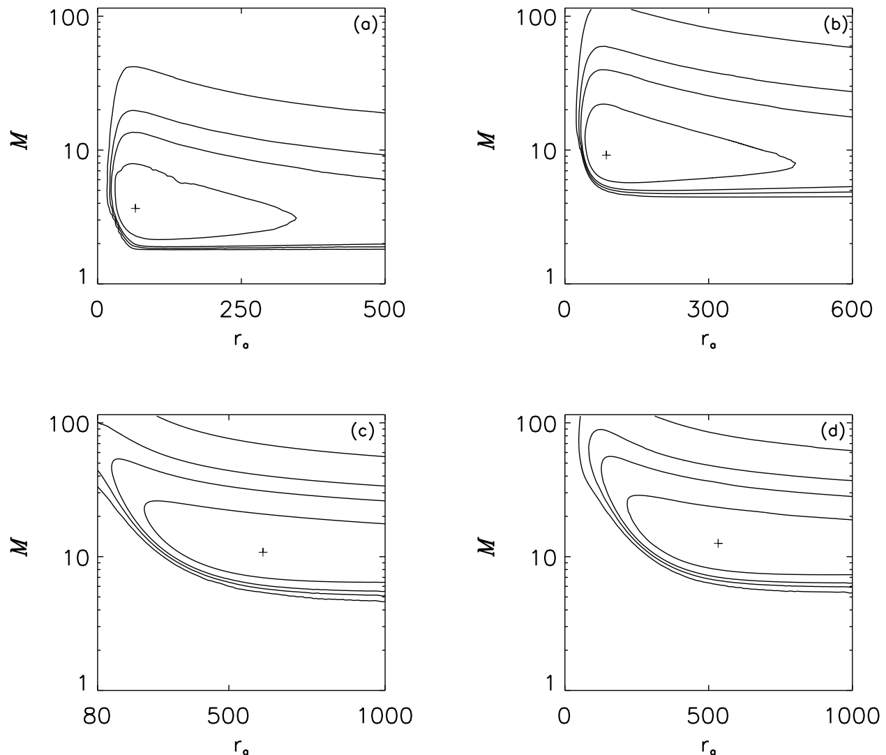
Figure 6. Likelihood contours for the total mass M (in units of 10^{11}M_{\odot} ) and the anisotropy radius r_a (in kpc). Contours are at heights of 0.32, 0.1, 0.045 and 0.01 of peak height. Data used: (a) Planetary nebulae only, (b) Globular clusters only, (c) Satellite galaxies only, (d) All data combined.
