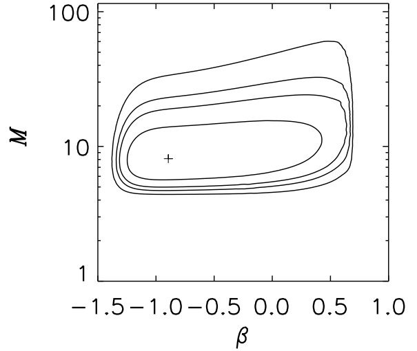
Figure 5. Likelihood contours for the total mass M (in units of 10^{11}M_{\odot} ) and the anisotropy parameter \beta , assuming a DF of the form (6). Contours are at heights of 0.32, 0.1, 0.045 and 0.01 of peak height. Data on the satellite galaxies only have been used.
