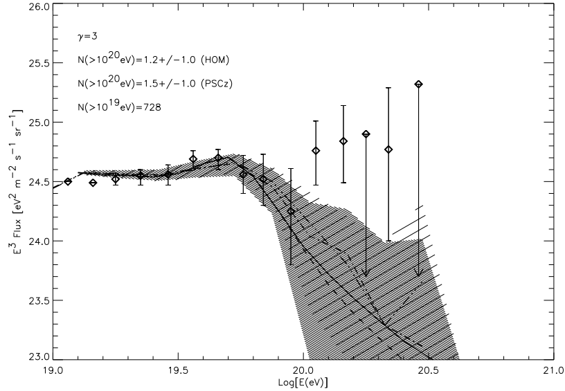
FIGURE 1. Simulated fluxes for the AGASA statistics of 728 events above 10^{19} eV, and \gamma = 3 , using a homogeneous source distribution (\ / hatches) and the PSCz distribution (dense / hatches). The solid and dashed lines are the results of the analytical calculations for the same two cases. The dash-dotted and dash-dot-dot-dotted lines trace the mean simulated fluxes for the homogeneous and the PSCz cases. (see [7]).
