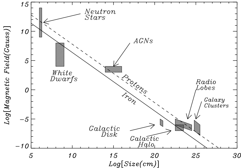
FIGURE 4. B vs. L , for E_{\text{max}} = 10^{20} eV, Z = 1 (dashed line) and Z = 26 (solid line) from [14].
