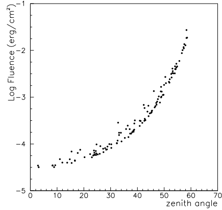
Fig. 4. – Upper limits on the energy fluence in the 1 GeV-1 TeV energy interval for 125 GRBs, in a time window \Delta t=10 s starting from the onset of the burst, as a function of the zenith angle of the event.
