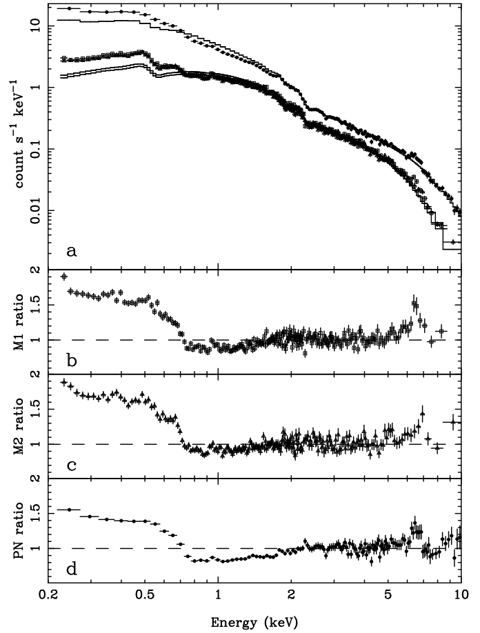
Fig. 1. a: spectra from MOS1 (open squares), MOS2 (open triangles), PN (filled dots) and power laws convolved with the instrument response functions (stepped lines). b,c,d: ratios of MOS1, MOS2, and PN spectra to the power law model.
