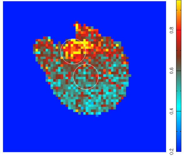
Fig. 3. EPIC-MOS \text{O}^{6+} / \text{O}^{7+} ratio image of N132D. The average ratios in the circular regions ( 15'' radius) are 0.79 \pm 0.01 near the northeastern rim and 0.60 \pm 0.01 in the centre.
