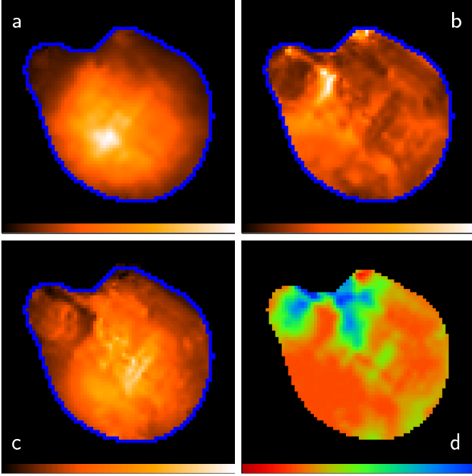
Fig. 4. N132D 150'' \times 150'' maps of (a) the Fe-K line flux at 6.67 keV, (range 0 - 1.66 \cdot 10^{-5} photons \text{cm}^{-2} \text{s}^{-1} \text{arcmin}^{-2} ), (b) the EW of the Fe-K line, (0 - 4.7 keV), (c) the differential continuum flux at 6.67 keV derived from the 4.4 - 10 keV spectrum, (0 - 1.15 \cdot 10^{-5} photons \text{cm}^{-2} \text{s}^{-1} \text{keV}^{-1} \text{arcmin}^{-2} ), (d) the apparent temperature (0.4 - 3.1 keV) derived from the continuum only. All colour bars are linear.
