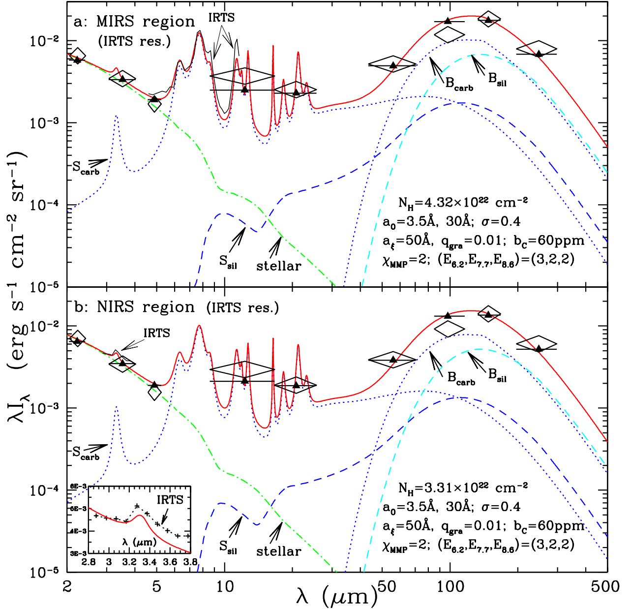
Fig. 10.— Infrared emission from dust plus starlight (see text) for two regions in the Galactic plane: (a) the MIRS region ( 44^{\circ} \leq l \leq 44^{\circ}40' , -0^{\circ}40' \leq b \leq 0^{\circ} ), and (b) the NIRS region ( 47^{\circ}30' \leq l \leq 48^{\circ} , |b| \leq 15' ). For both regions we use our standard dust parameters, with the PAH ionization fraction \phi_{\text{ion}} (a) taken to be the weighted mean for the local ISM (43% CNM, 43% WNM, 14% WIM). The starlight intensity heating the dust has been taken to be \chi_{\text{MMP}} = 2 . The solid curve shows the overall model spectrum, degraded to the IRTS resolution; triangles show the model spectrum convolved with the DIRBE filters. DIRBE observations are shown as diamonds. For the MIRS field we show the IRTS MIRS 5–12 \mu\text{m} spectrum (thin solid line). For the NIRS field we show the IRTS NIRS 2.8–3.9 \mu\text{m} spectrum (thin solid line, also shown as cross-dotted curve in inset). Curves labelled B_{\text{sil}} and B_{\text{carb}} show emission from “big” ( a \geq 250 \text{ \AA} ) silicate and carbonaceous grains; curves labelled S_{\text{sil}} and S_{\text{carb}} show emission from “small” ( a < 250 \text{ \AA} ) silicate and carbonaceous grains (including PAHs).
