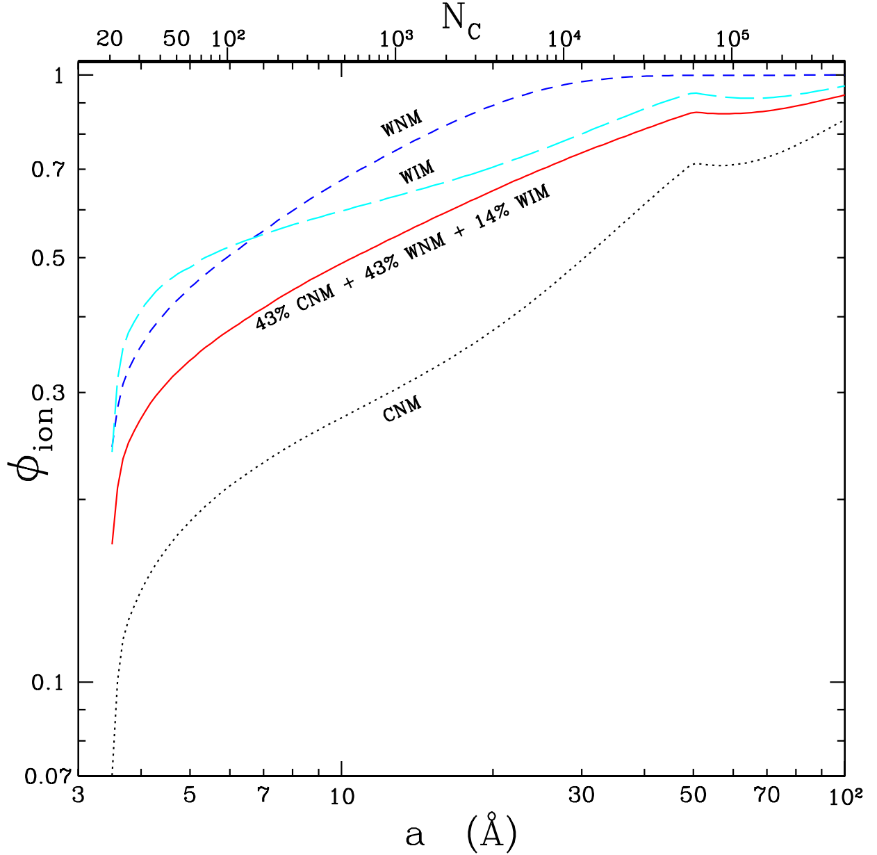
Fig. 7.— The “ionization fraction” \phi_{ion} – the probability of finding a PAH molecule in a non-zero charge state – as a function of size for three idealized phases of the diffuse ISM: CNM (dotted), WNM (short-dashed), and WIM (long-dashed). Solid line shows the averaged ionization fraction weighted by the mass fractions of Table 2. The slope discontinuity at a = 50 \text{\AA} is due to the transition from PAH optical properties to graphite properties above a_{\xi} = 50 \text{\AA} . The upper axis label give the number of carbon atoms N_C = 0.468(a/\text{\AA})^3 .
