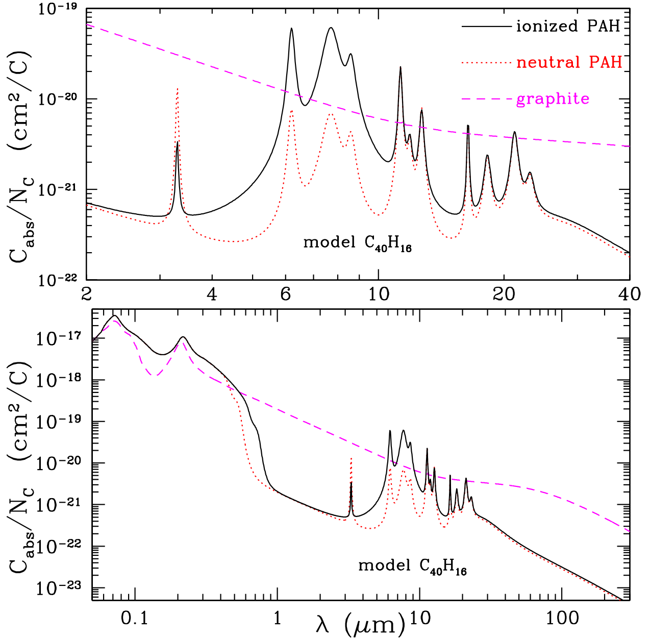
Fig. 2.— Absorption cross section per C atom of neutral and ionized PAHs (with E_{6.2}=3 , E_{7.7}=2 , E_{8.6}=2 ). Ionization enhances the C-C stretching modes ( 6.2 , 7.7 \mu\text{m} ) and C-H in-plane bending mode ( 8.6 \mu\text{m} ), and weakens the C-H stretching mode ( 3.3 \mu\text{m} ). Ionization shifts the visual absorption edge (which is also size-dependent) redward. The absorption cross section per C atom of small graphite spheres is shown for comparison.
