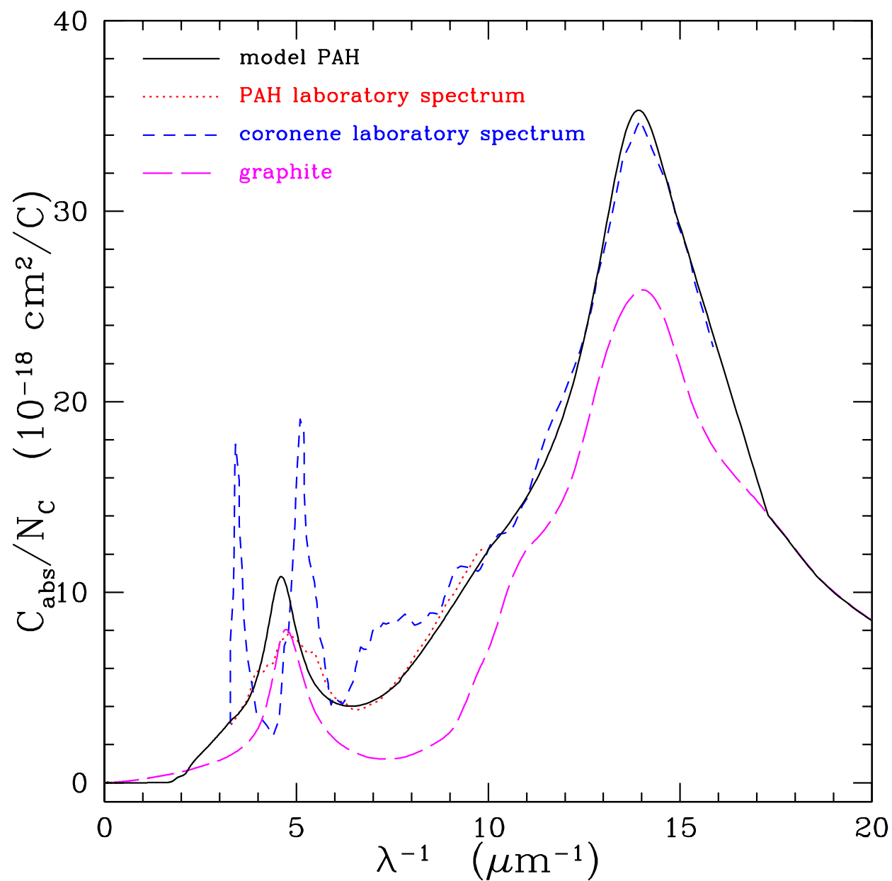
Fig. 1.— The ultraviolet and far ultraviolet absorption cross section per C atom of PAHs.
