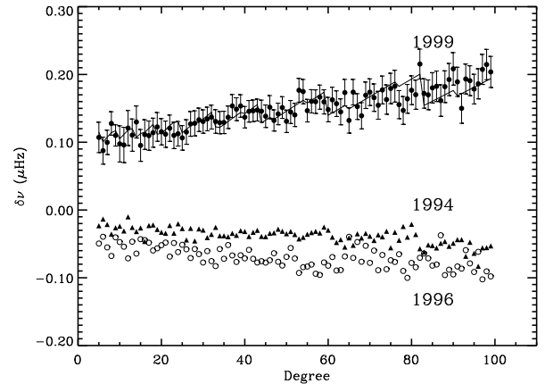
Figure 3. l -dependence of the frequency shifts for three different years. The solid line through the results corresponding to 1999, denotes the best linear fit to the inverse mode mass.
