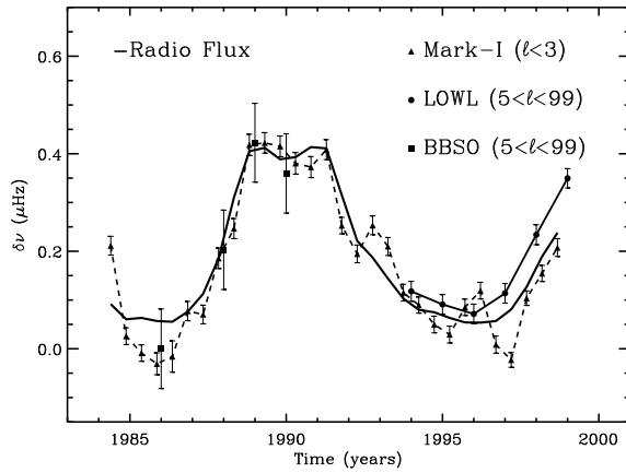
Figure 1. Time variation of the integrated frequency shift. The BBSO data have been averaged in the same way and plotted in the figure. In addition, 15 years of Mark-I frequency shifts are shown as well.
