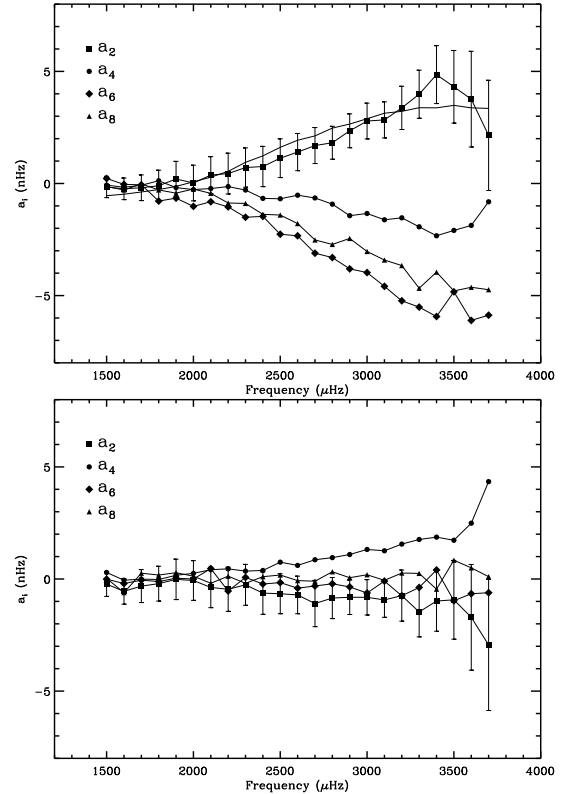
Figure 4. Frequency dependence of the even a -coefficients for two different years, 1996 (bottom) and 1999 (top).
