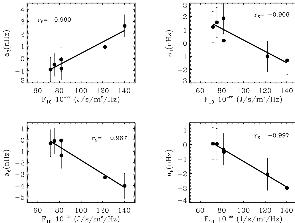
Figure 5. Variation of the integrated even a -coefficients against the radio flux at 10.7 cm. The solid line shows the best linear fit.
