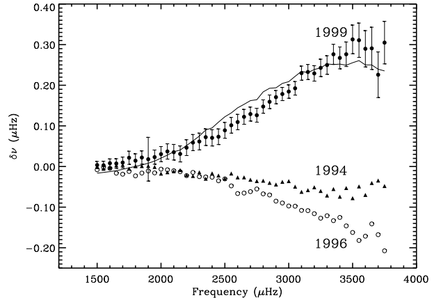
Figure 2. Frequency dependence of the frequency shift for three years. The error bars have been shown just for one year for clarity. The solid line represents the best linear fit of the inverse mode mass to the 1999 observations.
