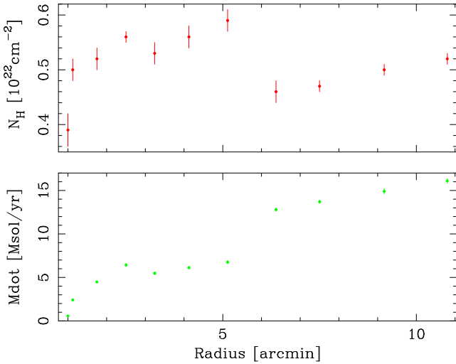
Fig. 14. Results of a cooling flow analysis in concentric circles around M87 (using MOS1). Shown are the parameters for the warm absorption hydrogen column density in the cooling flow and the inferred mass flow rate (for details see text).
