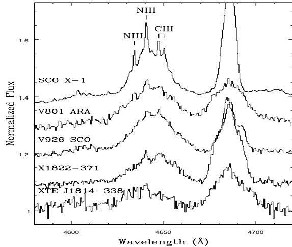
Fig. 3. Doppler-corrected sums, in the rest frame of the companion, of systems studied by our group so far.
