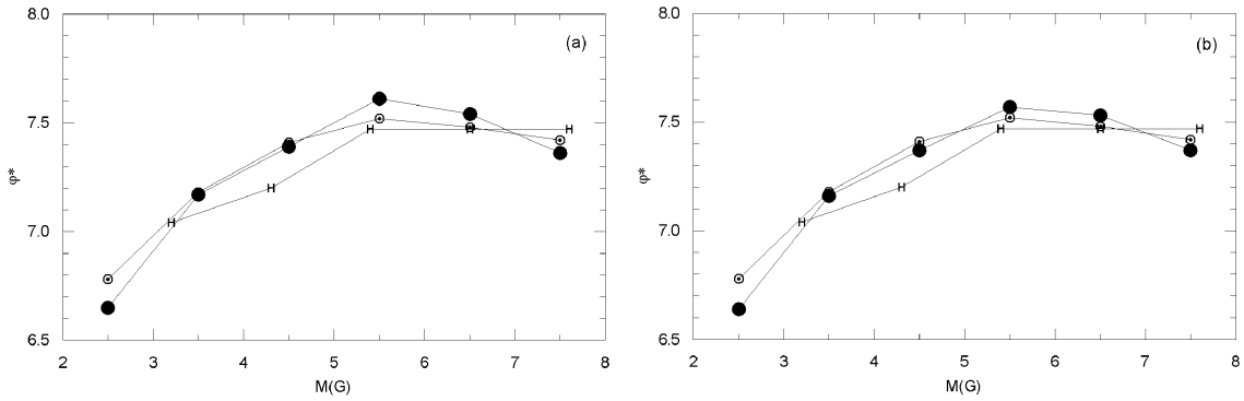
Figure 7: Logarithmic stellar luminosity function, implied by two model-gradients: (a) GW, and (b) BRK ( \bullet ) confronted to Gliese's (1969) ( \odot ), and Hipparcos' (JW 1997) (H) values.
