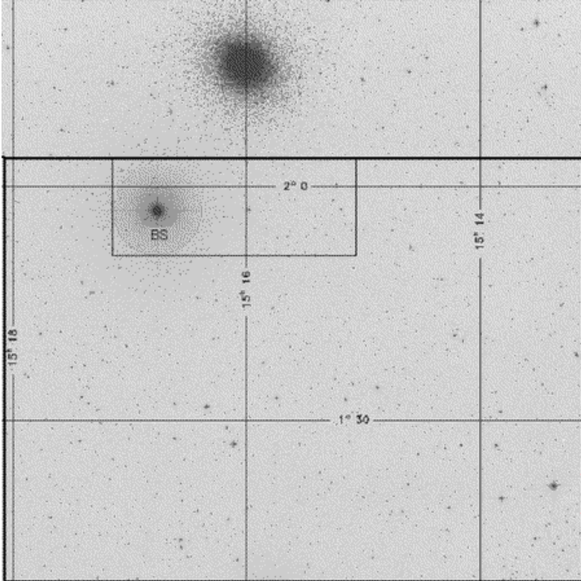
Figure 2: The field chart showing the position of the cluster M5, the bright star HD 136202 ( \alpha = 15^h 19^m 18^s.80 , \delta = +01^\circ 45' 55''.5 ), labelled with BS, and the surrounding excluded area of 0.104 square-degrees. The horizontal and vertical axes give the right ascension ( \alpha ) and declination ( \delta ), respectively.
