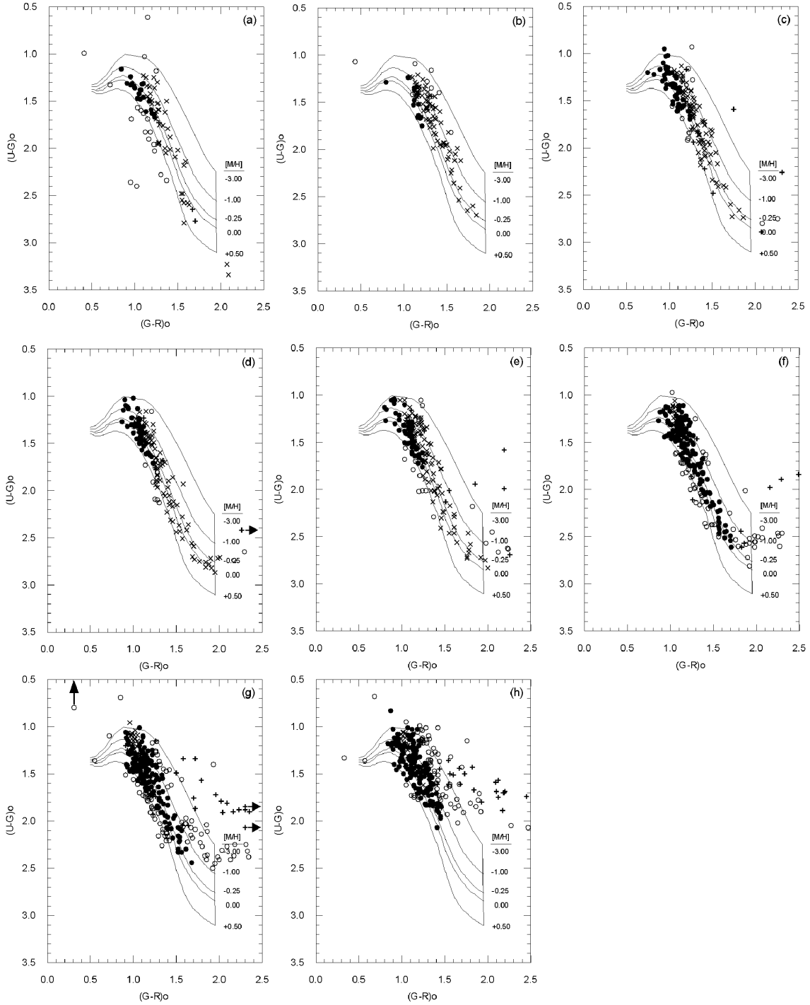
Figure 4: Two-colour diagrams in consecutive apparent magnitude intervals, i.e. (a) G \leq 14.0 , (b) 14.0 < G \leq 15.0 , (c) 15.0 < G \leq 16.0 , (d) 16.0 < G \leq 16.5 , (e) 16.5 < G \leq 17.0 , (f) 17.0 < G \leq 17.5 , (g) 17.5 < G \leq 18.0 , and (h) 18.0 < G \leq 18.5 . The superposed grid of iso-metallicity lines for dwarf stars is based on theoretical model atmosphere calculations (Buser & Fenkart 1990). Symbols: ( \bullet ) dwarf, ( \times ) evolved, ( \circ ) untreated, and ( + ) extra-galactic objects.
