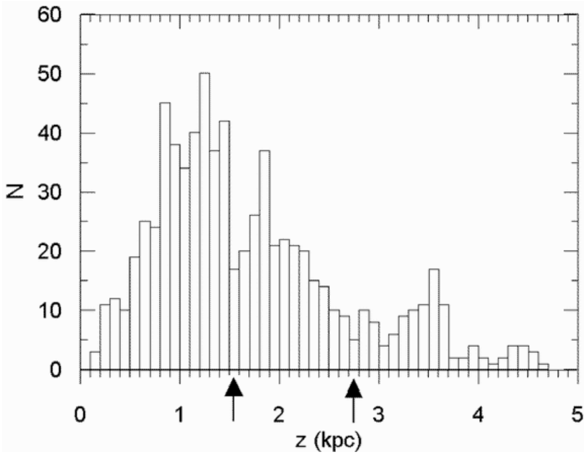
Figure 10: The spatial distribution for dwarfs and sub-giants within the limiting distance of completeness. The distances to the Galactic plane z = 1.6 kpc and z = 2.75 kpc (shown by arrows) are the borders of three populations, Population I (thin disk), Intermediate Population II (thick disk), and Extreme Population II (halo).
