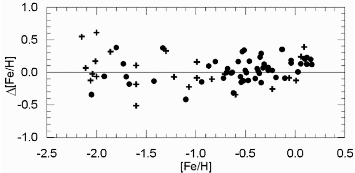
Figure 13: \Delta[Fe/H] versus metallicity, where \Delta[Fe/H] is the difference between the original metallicities and the evaluated ones, utilising the new calibration, [Fe/H] = 0.11 - 2.22\delta_{1.08} - 7.95\delta_{1.08}^2 . Symbols: (●) stars from Carney (1979), and (+) stars from Cayrel de Strobel et al. (1997).
