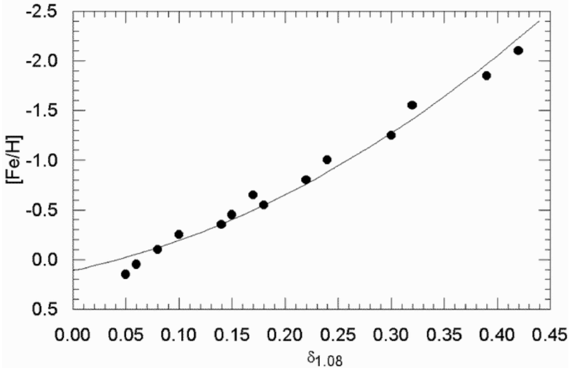
Figure 12: [Fe/H] metallicity versus normalized \delta_{1.08} ultra-violet excess for RGU photometry.
