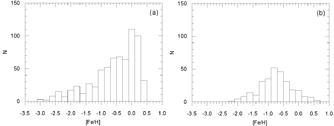
Figure 8: The metallicity distribution for dwarfs (a) and sub-giants (b).
