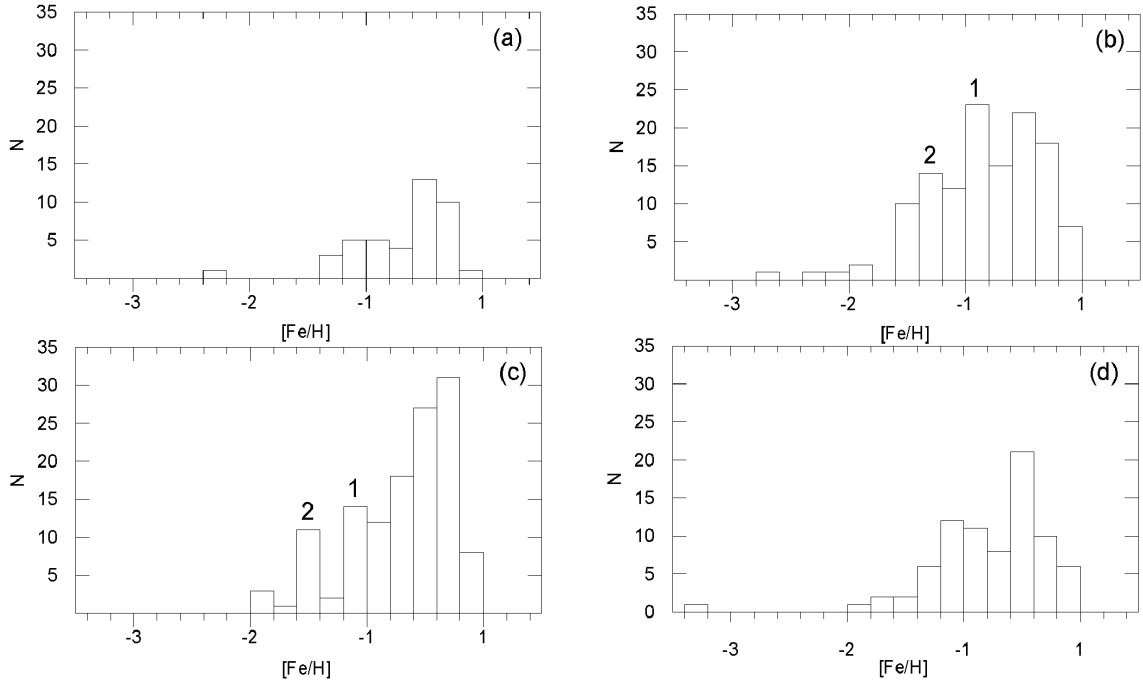
Figure 9: Metallicity distribution for dwarfs (only) with 4 < M(G) \leq 6 mag, corresponding to spectral types F5-K0, for four z -intervals: (a) 0 < z \leq 0.75 , (b) 0.75 < z \leq 1.5 , (c) 1.5 < z \leq 2.5 , and (d) 2.5 < z \leq 4 kpc. The comparison of Fig.9b and 9c reveals a metallicity gradient of d[Fe/H]/dz = -0.20 dex/kpc.
