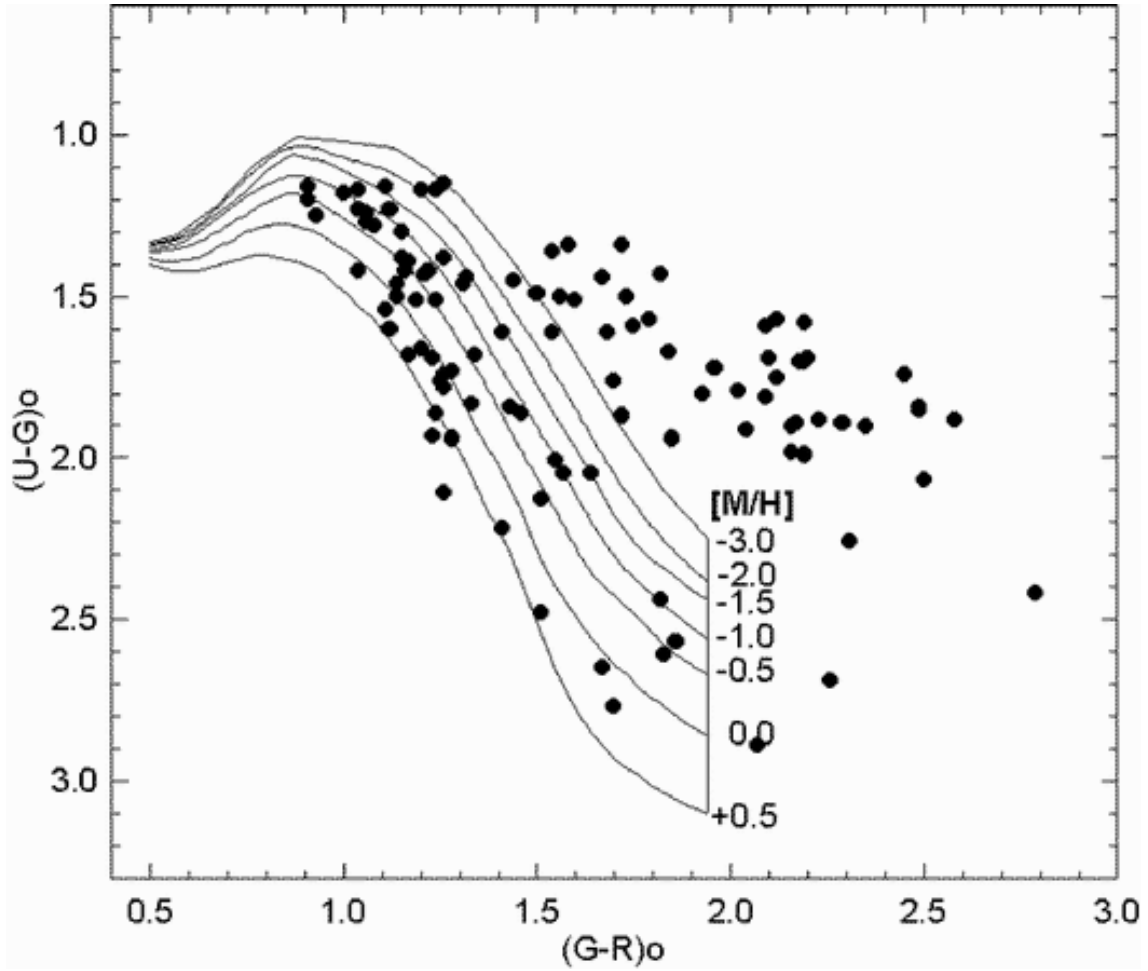
Figure 1: Extra-galactic objects identified by comparison of Minnesota and Basel charts. Their number within the limiting apparent magnitude, G = 18.5 , is 104, but increases up to 164 when counted down to the faintest object in the Basel catalogue.
