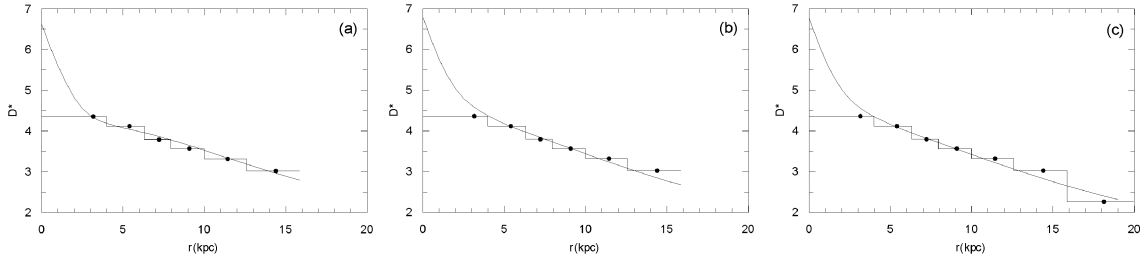
Figure 6: Logarithmic space-density histograms for giants for all populations ( M(G) \leq 2 mag), within the limiting apparent magnitude. ( \bullet ) centroid-distance within the limiting distance of completeness for comparison with two model gradients, i.e. (a) GW, (b) BRK, and (c) BRK for a larger distance interval ( r \leq 19.95 kpc).
