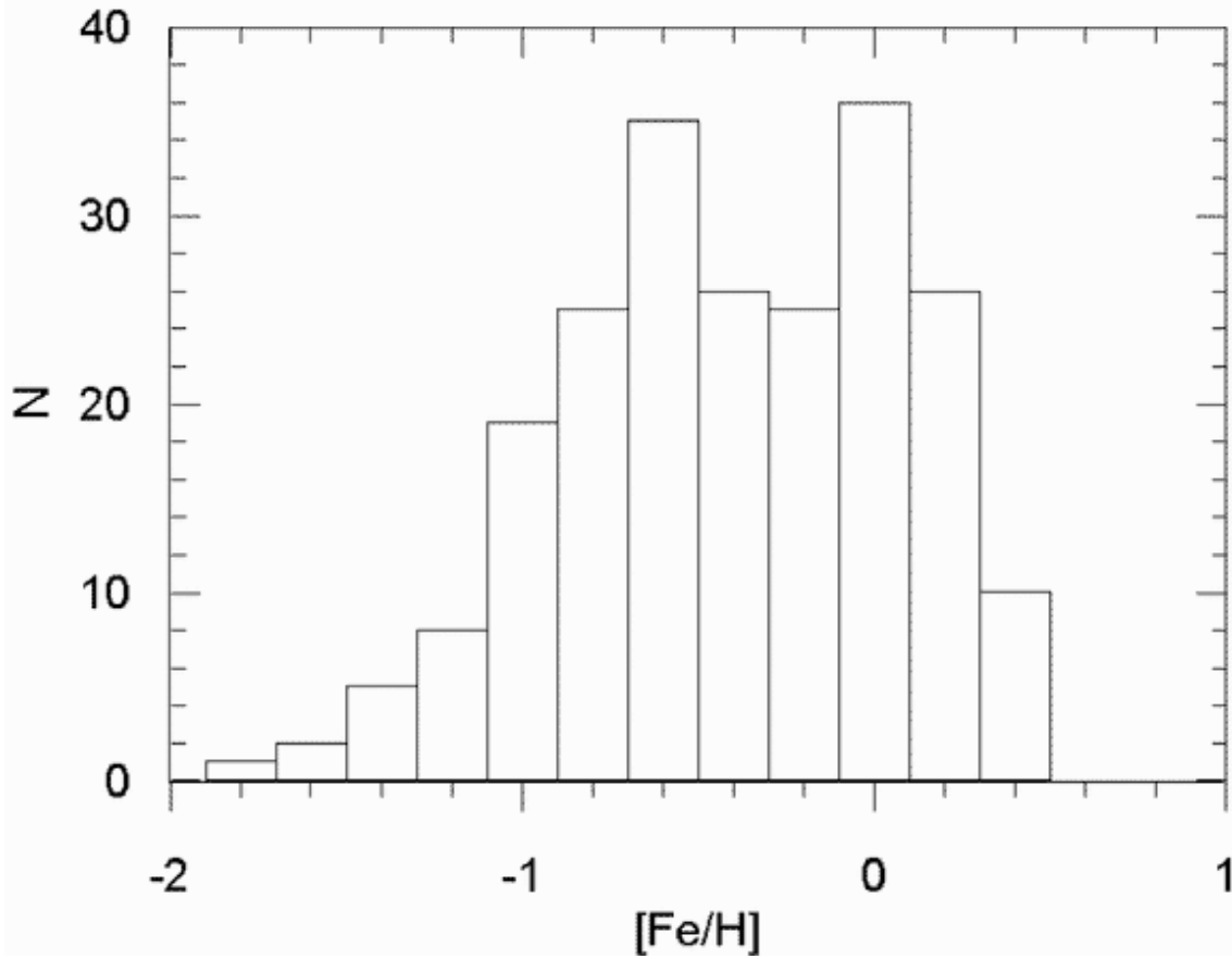
Figure 11: The metallicity distribution for dwarfs and sub-giants with 1.6 < z \leq 2.75 kpc, i.e. for the thick disk, giving a bimodal distribution. The first mode at [Fe/H] = -0.63 dex corresponds to the canonical metal abundance assigned to the thick disk (Gilmore & Wyse 1985, Wyse & Gilmore 1986, Buser et al. 1999, and Rong et al. 2001), and the second at [Fe/H] = +0.06 dex to the metallicity cited for the same component of the Galaxy very recently (Carney 2000, Karaali et al. 2000).
