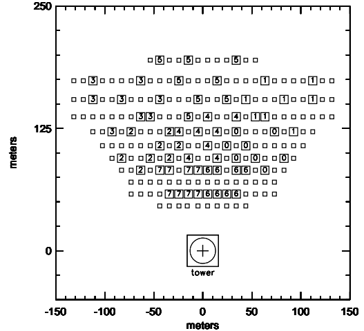
FIG. 1.— Map of the heliostat field used by the STACEE experiment, showing updates to the experiment over time. Heliostats are numbered according to the trigger subcluster to which they belong. Clusters 0, 1, 2, and 3 correspond to the “east” and “west” cameras; most of these heliostats were used in the STACEE-32 prototype. Clusters 4 and 5 correspond to the “north” camera which was added for STACEE-48. Clusters 6 and 7 correspond to the new STACEE-64 “southeast” and “southwest” cameras. The base of the NSTTF solar tower, which houses the STACEE optics and electronics, marks the origin of the coordinate system.
