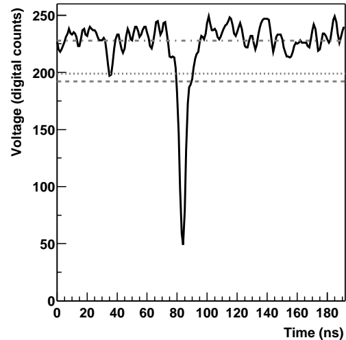
FIG. 2.— Digitized PMT signal from a typical air shower event. Dot-dash line: FADC baseline. Dashed line: Discriminator threshold. Dotted line: 3 standard deviations above baseline for NSB fluctuations.
