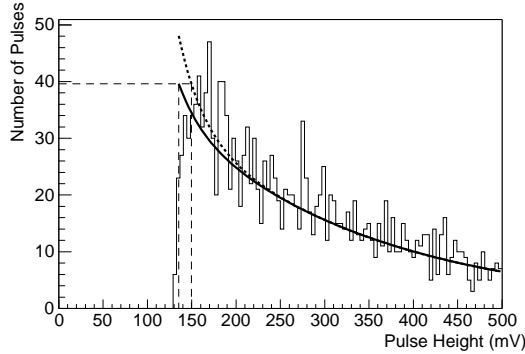
FIG. 5.— Pulse height distribution of triggered events from a 10-minute segment of a typical OFF-source run on the star \iota CrB. The best-fit form of a Poisson distribution (expected NSB) plus an exponential is shown (solid line), as well as the predicted form for the ON-source run (dashed line) resulting from additional NSB fluctuations. The ON-source prediction is normalized to the same detector livetime as the OFF-source best fit. Horizontal dashed line: number of OFF-source pulses per mV at the nominal hardware discriminator threshold. Vertical dashed lines: analysis thresholds ON and OFF necessary to equalize the number of pulses above threshold over the course of the run.
