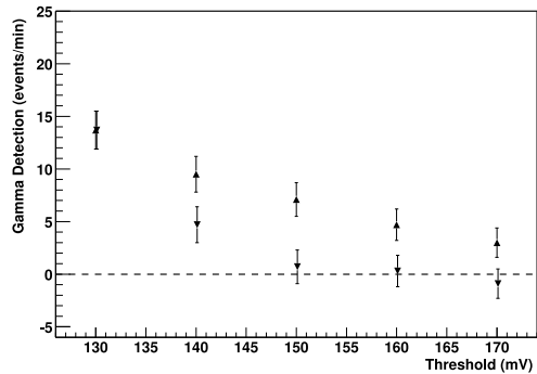
FIG. 4.— Excess event trigger rate as a function of FADC analysis threshold in the library padding analysis of a subset of data taken on the star \iota CrB. The trigger condition is described in the text. Upright triangles: No padding of traces before retriggering. Inverted triangles: Traces are padded to equalize RMS before retriggering. Dashed line: zero promotion excess. The figure shows that the minimum threshold necessary to remove all hadronic promotion events from the library-padded data set is 150 mV.
