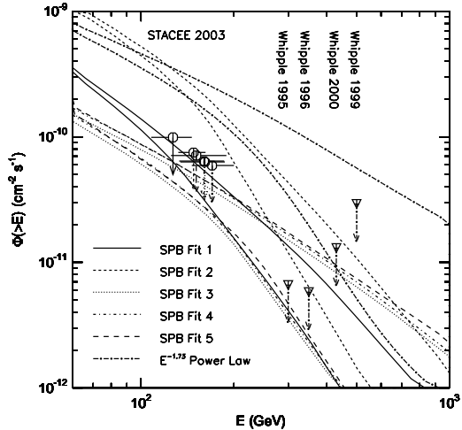
FIG. 7.— Integral flux in \text{cm}^{-2} \text{s}^{-1} for each of the five SPB models from Boettcher, Mukherjee & Reimer (2002), and for the extrapolation of the best-fit EGRET power law (Hartman et al. 1999). Model predictions for both low and high EBL optical depth are shown, along with STACEE upper limits for mean EBL optical depth. Upper limits from observations with the Whipple 10-meter from 1995–2000 are also shown (Horan et al. 2003).
