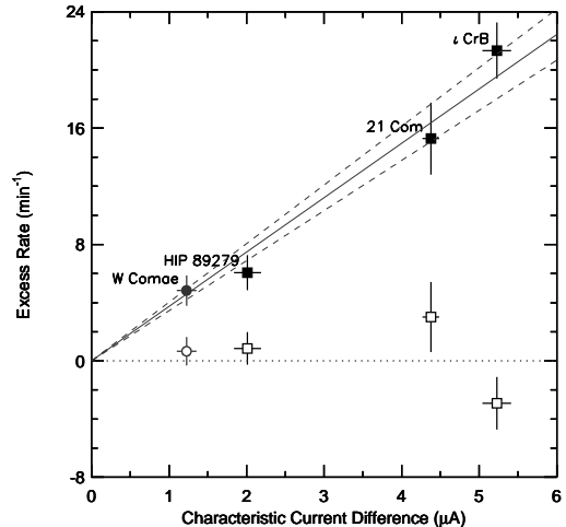
FIG. 3.— Excess event trigger rates as a function of the characteristic current difference for sources observed in 2002–2003 by STACEE-64. Squares: star observations; circle: W Comae. Filled symbols show the raw excess, and open symbols show the excess after the dynamic threshold brightness correction. The lines show the best-fit linear trend constrained to go through the origin (solid) with 68% confidence errors on the slope (dashed), and the zero-rate baseline (dotted).
